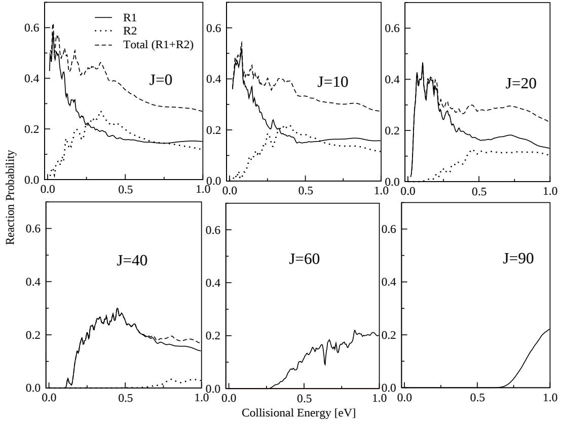
Figure 4.1: The probability of \text{H} + \text{LiH}^+ ( v=0, j=0 ) reaction as a function of collision energy. The probabilities of R1 and R2 channel are shown by the solid and dotted lines, respectively. The dashed line indicate the total probability of the \text{H} + \text{LiH}^+ reaction.
