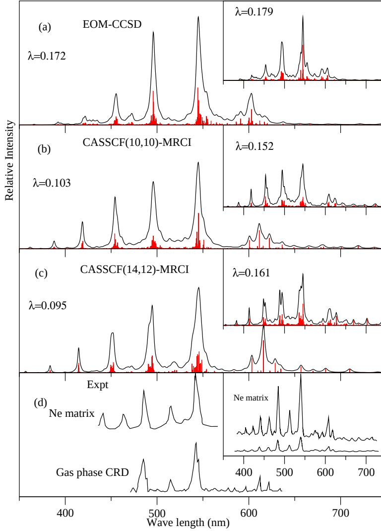
Figure 3.6: The \tilde{B}^1B_1 \leftarrow \tilde{X}^1A_1 absorption spectrum of l-C 3 H 2 calculated with the EOM-CCSD (panel a), CASSCF(10,10)-MRCI (panel b) and CASSCF(14,12)-MRCI (panel c) electronic structure results (see text for details). The experimental results of Maier et al. [7] and presented in panel d. The experimental results of Hodges et al. [6] given in the inset of panel d.
