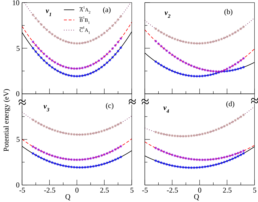
Figure 3.1: Adiabatic potential energy of first three excited electronic states of l-C 3 H 2 along the normal displacement coordinates of the totally symmetric vibrational modes. The points in the figure represent calculated EOM-CCSD energies and the lines connecting them are the adiabatic potential energy functions derived from the diabatic electronic Hamiltonian.
