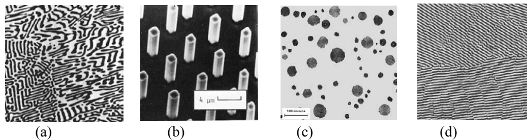
Figure 1.12 Various microstructures in eutectic systems. a) Irregular microstructure in Mg-Mg 2 Sn eutectic. The dark phase is the faceted Mg 2 Sn, b) Rod shaped faceted/non-faceted microstructure in Ni-NbC eutectic, c) Divorced microstructure in Fe-spheroidal graphite eutectic, d) Lamellar arrangement in Sn-Pb system(adapted from ref.66d).
