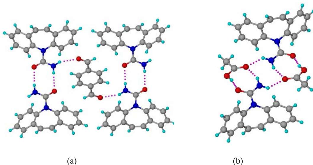
Figure 2.7a) The prominent amide-amide homodimer of CBZ guest free form is retained in the CBZ-Terephthaldehyde cocrystal. b) While amide-Acid Heterosynthon is preferred in the CBZ-Acetic acid cocrystal. (Adapted from ref.11d)
