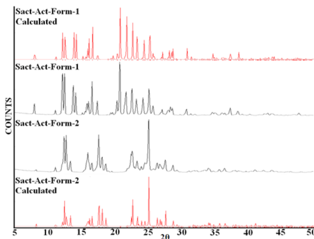
Figure 4.11a) Overlay of experimental PXRD pattern of SACT-ACT form 1 (2 nd from top) with the experimental PXRD matching with form 2, obtained after slurry grinding in toluene for 2 days (3 rd from top). The respective calculated patterns of form 1 and 2 (top and bottom) are shown for comparison.
