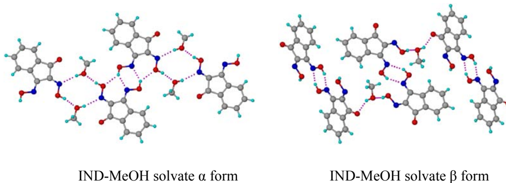
Figure 1.7 In \alpha form guest molecules bridge the dimeric units of IND through O–H \cdots N and O–H \cdots O hydrogen bonds resulting in the centrosymmetric cyclic assembly. In \beta form dimeric units of IND are linked by a single MeOH molecule extending the assembly through O–H \cdots O hydrogen bonds (adapted from ref.52c).
