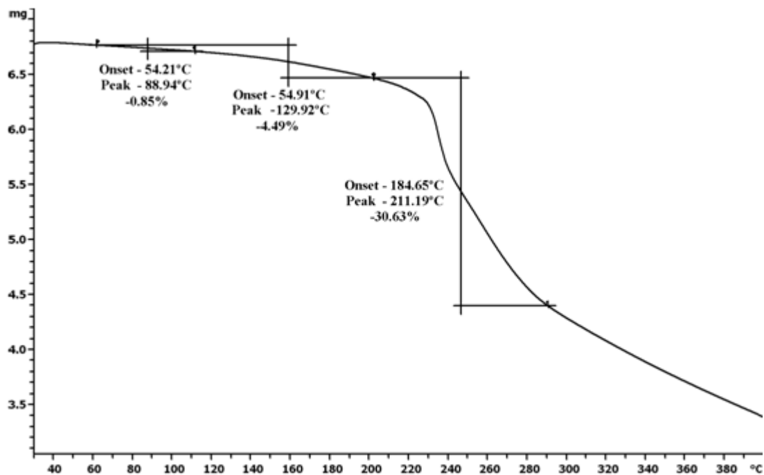
Figure 2.11 TGA curve of FUROS-BPNO-0.25H 2 O. The weight loss of 0.85% between 60-90 °C accounts for the loss of \frac{1}{4} water molecule. The major decomposition of cocrystal components occur between 120-300 °C.
