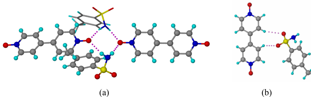
Figure 2.4a) Tetrameric R^2_4(8) rings of \text{N-H}\cdots\text{O} hydrogen bonds between PTS and BPNO molecules. Symmetry-independent PTS molecules are shown as capped-stick and ball-stick models. b) \text{C-H}\cdots\text{O} synthon of R^2_2(9) motif in the crystal structure.
