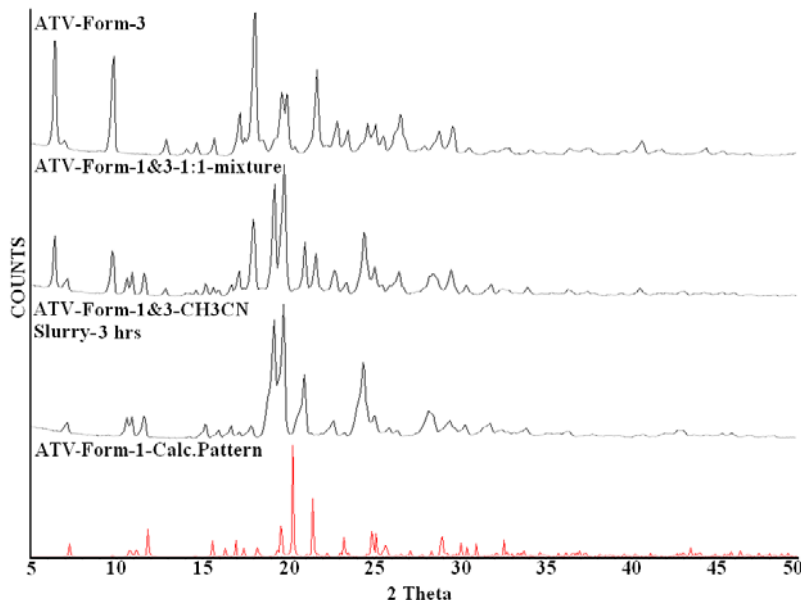
Figure 7.13e) Overlay of experimental PXRD pattern of 1:1 mixture of ATV form 1 and 3 (2 nd form top) with the experimental PXRD matching with form 1, obtained after slurry grinding the mixture in CH 3 CN for 3 hrs (3 rd form top). The experimental pattern of form 3 (top) and the calculated pattern of form 1 are shown for comparison (bottom).
