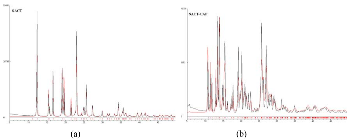
Figure 6.13a) Representative PXRD pattern of SACT, SACT-INIC and SACT-THEO at the end of equilibrium solubility and dissolution experiments matches very well with SACT when overlayed with its calculated pattern. b) Representative PXRD pattern of SACT-CAF at the end of equilibrium solubility and dissolution experiments matches very well with its calculated pattern indicating phase stability.
