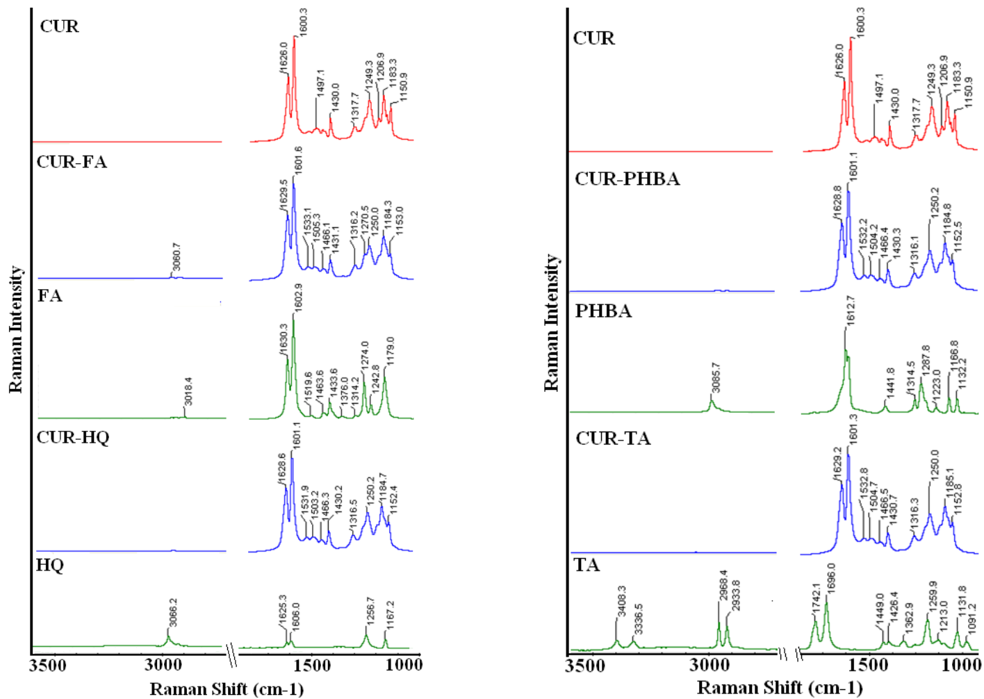
Figure 5.9 Raman spectra of curcumin eutectic compositions overlayed with their starting components.
