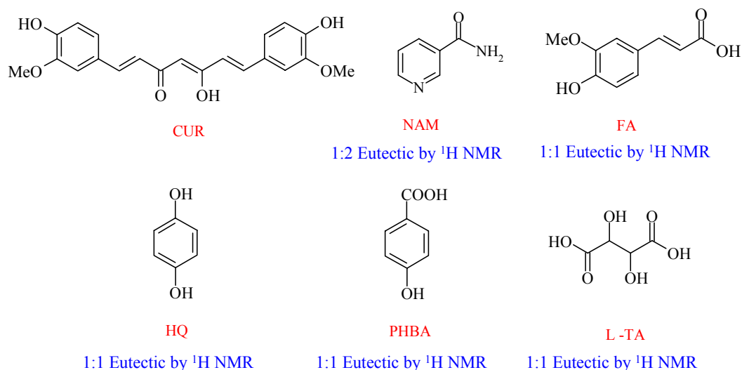
Scheme 5.1 Curcumin and coformers discussed in this study. The stoichiometry of curcumin–coformer was determined by 1 H NMR and eutectic nature established by DSC.
