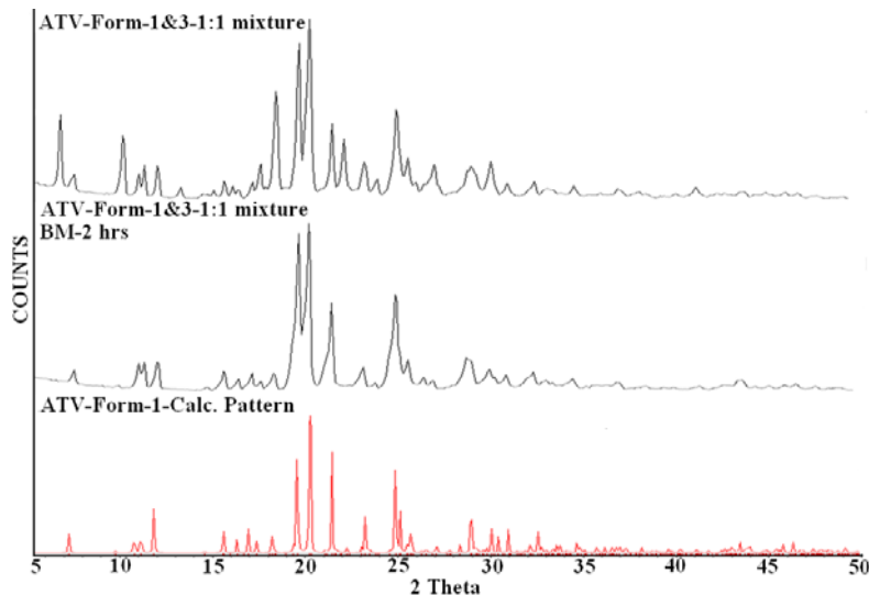
Figure 7.15e) Overlay of experimental PXRD pattern of 1:1 mixture of ATV form 1 and 3(top) with the experimental PXRD matching with form 1, obtained after ball mill grinding the mixture for 2 hrs (2 nd form top). The calculated pattern of form 1 is shown for comparison (bottom).
