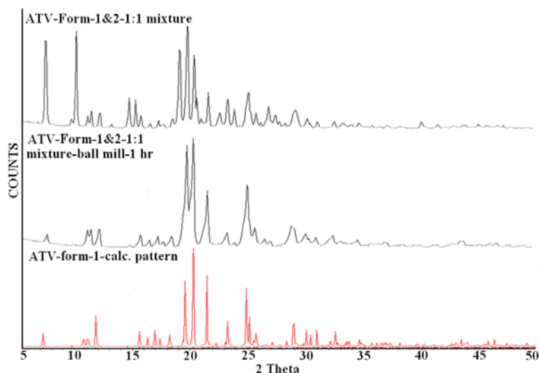
Figure 7.15d) Overlay of experimental PXRD pattern of 1:1 mixture of ATV form 1 and 2(top) with the experimental PXRD matching with form 1, obtained after ball mill grinding the mixture for 1 hr (2 nd form top). The calculated pattern of form 1 is shown for comparison (bottom).
