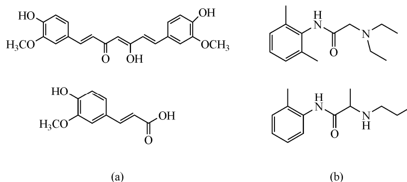
Scheme 5.3a) Molecular structures of curcumin and ferulic acid and b) lidocaine and prilocaine. The structural similarity between the components might have resulted in eutectic formation.
