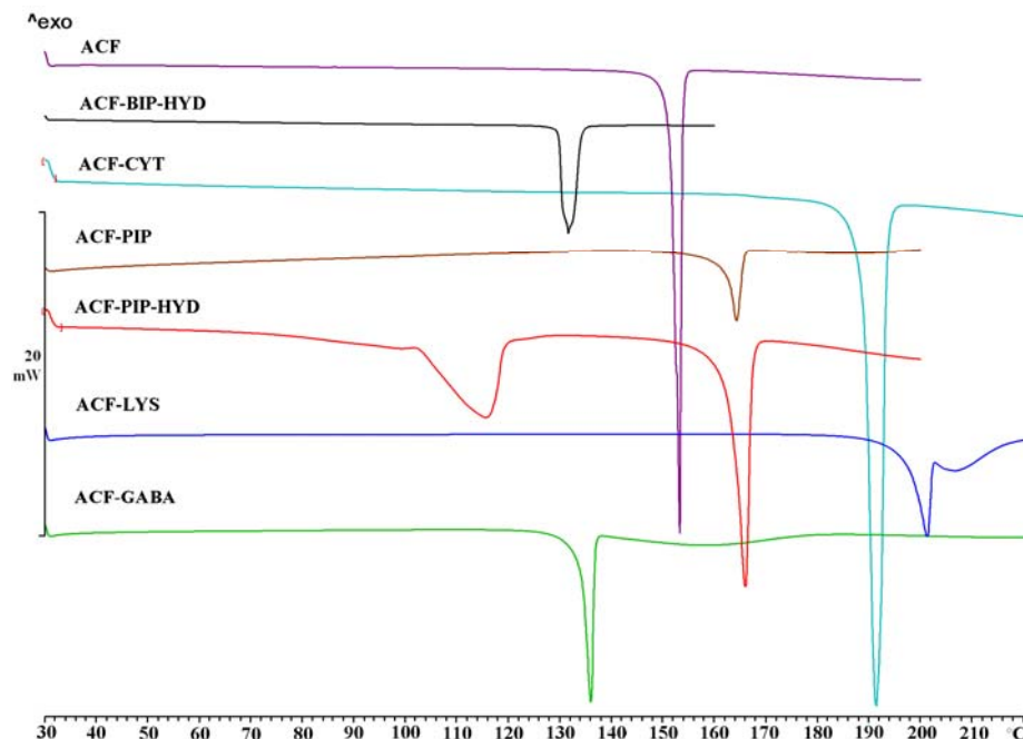
Figure 3.9 DSC heating curves show a sharp melting endotherm for each solid form.
