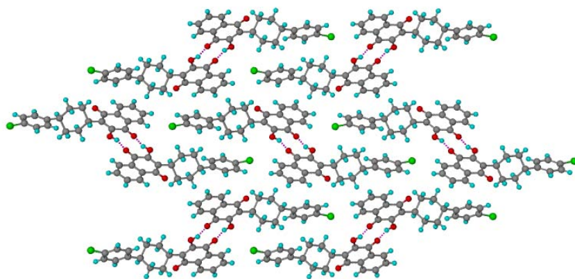
Figure 7.3b) Dimeric ATV molecules arranged in an anti-parallel fashion in the adjacent layers.
