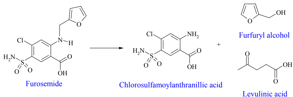
Scheme 2.4 Thermal degradation products of furosemide
