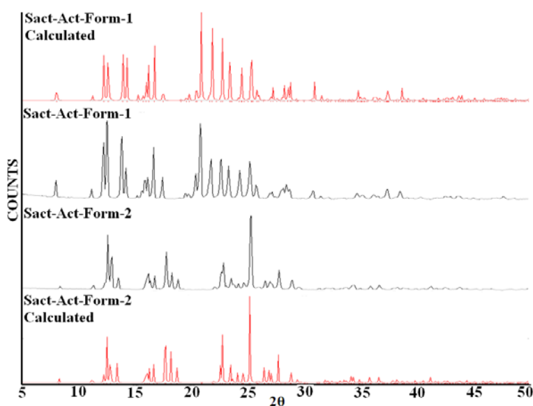
Figure 4.12a) Overlay of experimental PXRD pattern of SACT-ACT form 1(2 nd from top) with the experimental PXRD matching with form 2, obtained after neat grinding in ball mill for 30 min (3 rd from top). The respective calculated patterns of form 1 and 2 (top and bottom) are shown for comparison.
