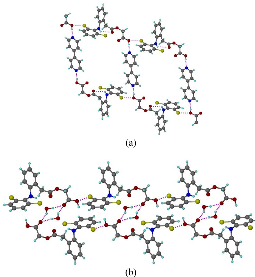
Figure 3.3a) ACF and BIP molecules are connected through O–H \cdots N hydrogen bond. b) Adjacent ACF layers are connected through water bridges in a tetramer O–H \cdots O motif.
