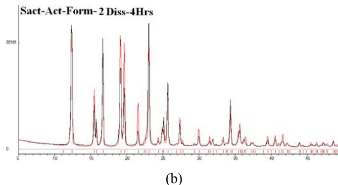
Figure 4.15 PXRD plots of SACT cocrystal polymorphs at the end of dissolution experiment matches with the calculated XRD pattern of SACT indicating form conversion. Similar phase transformation was observed at the end of solubility experiment on cocrystal polymorphs.
