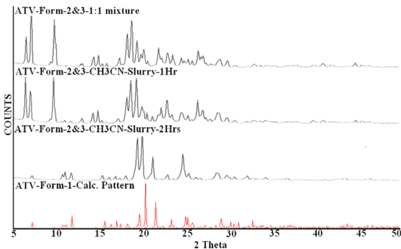
Figure 7.13f) Overlay of experimental PXRD pattern of 1:1 mixture of ATV form 2 and 3 (top) with the experimental PXRD matching with all three forms after 1hr (2 nd from top), converted completely to form 1 after 2 hrs (3 rd form top). The calculated pattern of form 1 (bottom) is shown for comparison.
