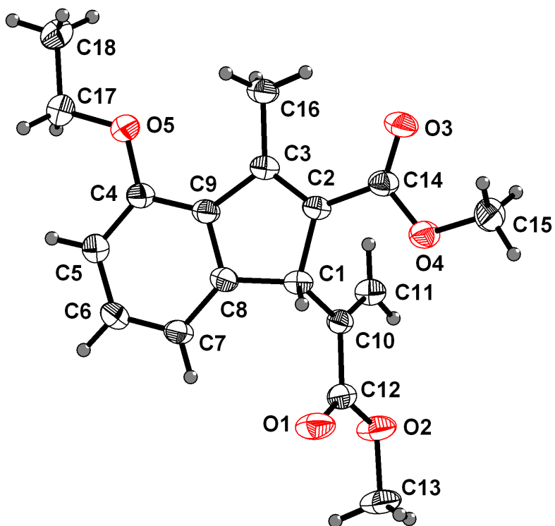
Fig. X7 ORTEP diagram of the compound ortho - 93k
