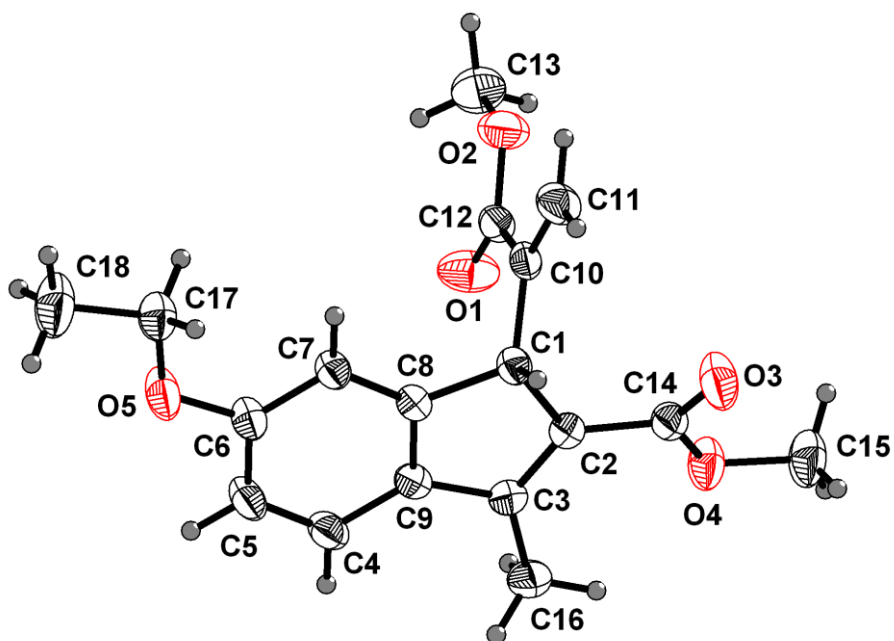
Fig. X6 ORTEP diagram of the compound 93k
