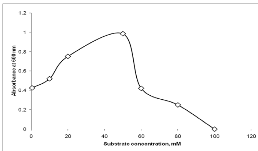
Fig. 3.1 Growth of strain DS004 at different concentrations of acephate.
