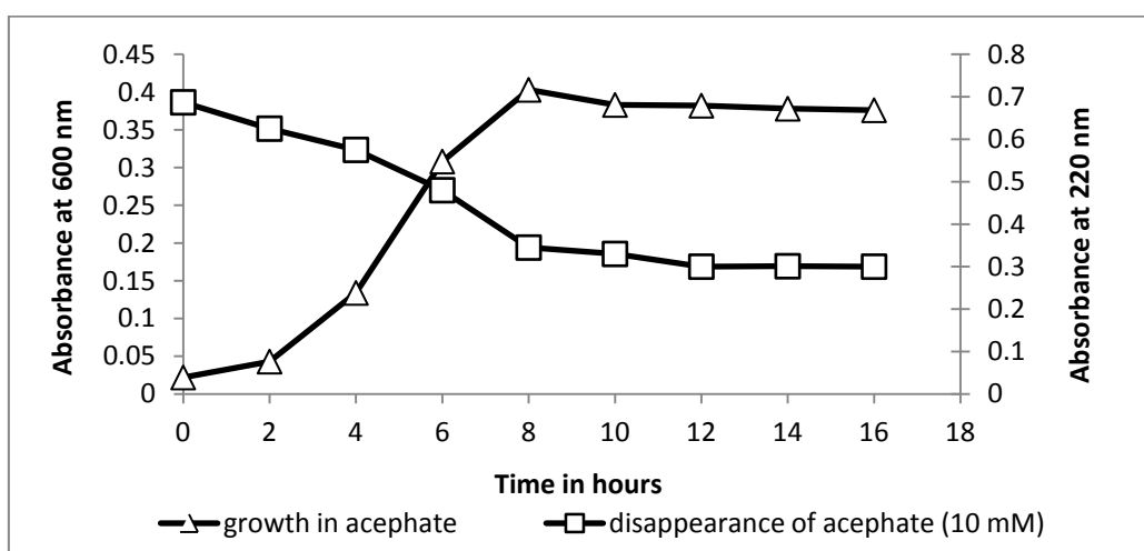
Fig. 3.2 Graph showing inverse relationship between growth of the strain DS004 and disappearance of acephate.
