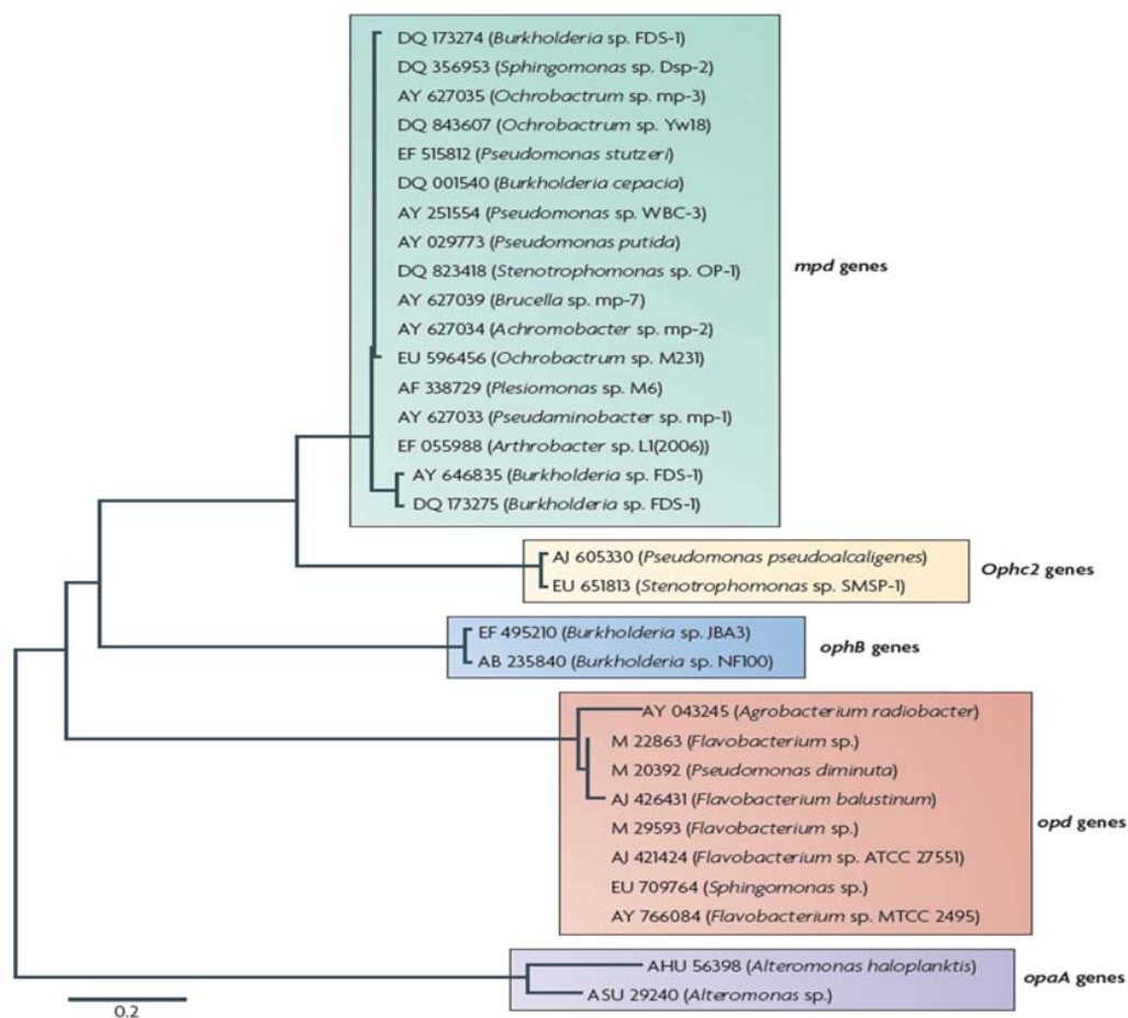
Fig. 4.12. Phylogenetic tree constructed from organophosphorus-degrading gene sequences. The tree was compiled using the sequences that were available in the NCBI database. Distinct groups that correspond to different genes, such as the mpd (methyl parathion degrading), opd (organophosphorus degrading) and opaA (organophosphorus acid anhydrolase) genes are easily delineated (shown in different colours). The tree was constructed using a neighbour-joining method and Mega4 software. All major nodes are supported by a bootstrap value of >50%. The scale bar represents the number of expected changes per site. The locus tags are provided for each gene followed by the species name in brackets (Singh, 2008).
