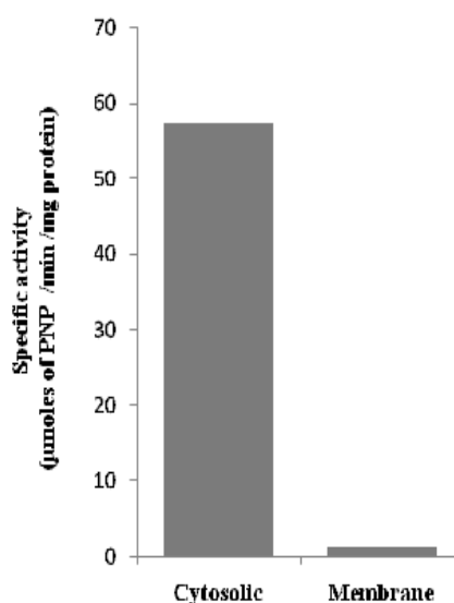
Fig. 5.14. OPH activity in subcellular fractions. The bar diagram represents OPH activity obtained in cytoplasmic and membrane fractions prepared from P.jinjuensis biotype acephalyticus (pHNSKMOPD).
