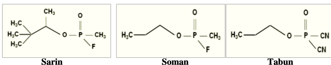
Fig.1.3. Chemical Structures of Nerve gases that belongs to organophosphate group.
