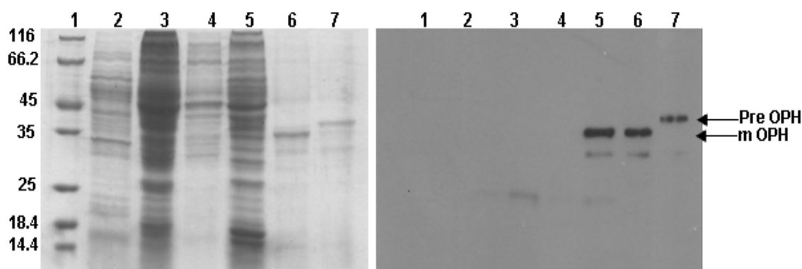
Fig. 5.13. Subcellular localization of preOPH in P.jinjuensis biotype acephalyticus (pHLCKMOPD). Panel A) SDS-PAGE analysis of subcellular fractions. Panel B represents corresponding western blots performed using anti-His antibody to detect OPH-6His. Lane 2 and 3 represent protein extracts prepared from cytoplasmic and membrane fractions prepared from wild type P.jinjuensis biotype acephalyticus . Lane 4 and 5 represent similar extracts prepared from strains containing expression plasmid pHLCKMOPD. Partially purified mOPH and preOPH used as size markers are loaded in lanes 6 and 7. The OPH specific signal corresponding to the size of mOPH is seen in lane 5.
