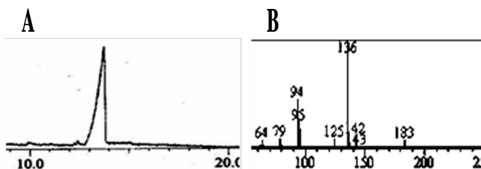
Fig. 4.1. Panel A shows gas chromatogram showing single peak of acephate with retention time 13.8 min. Panel B shows mass spectrum of acephate showing the presence of acephate with molecular mass 183.
