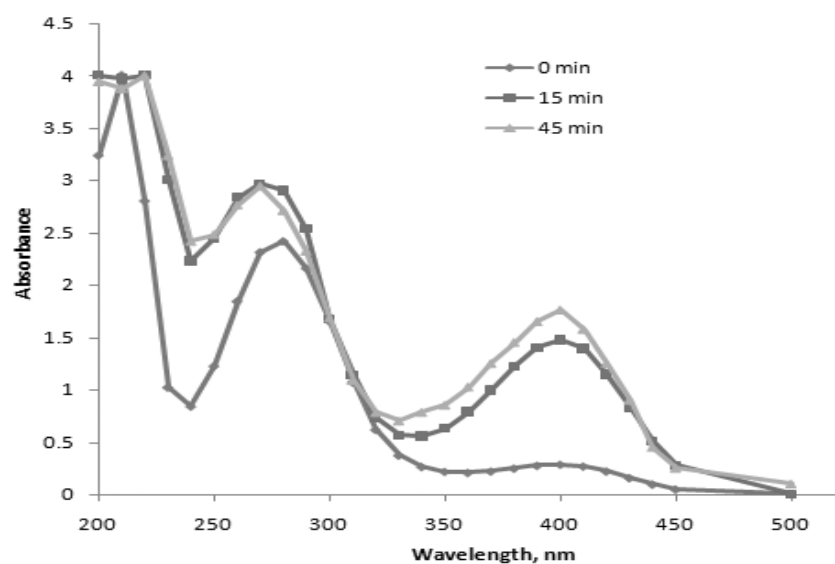
Fig. 5.16. Degradation of Parathion by Pseudomonas jinjuensis biotype acephalyticus expressing mOPH.
