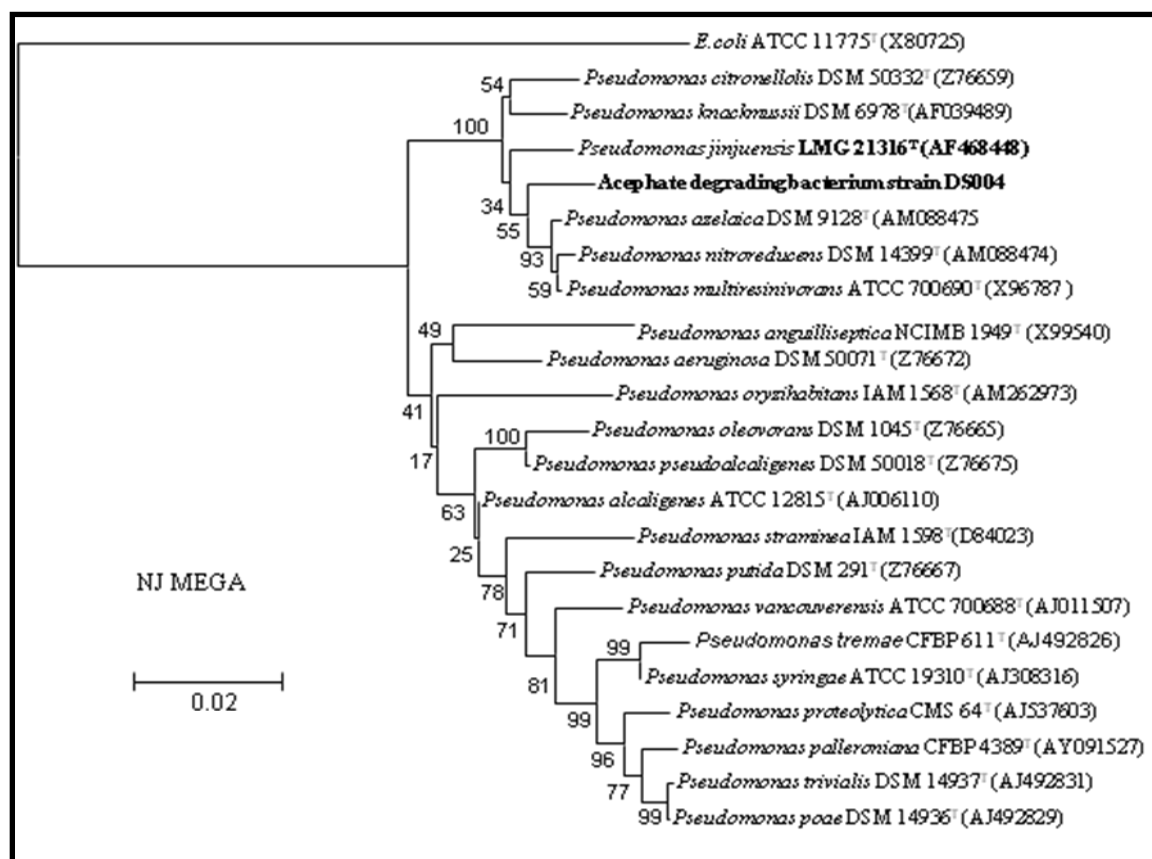
Fig. 3.11 Phylogenetic tree of strain DS004 constructed using 16S rRNA gene sequence.
