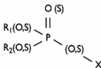
Fig.1.1 General formula of organophosphorus compounds where \text{R}_1 , \text{R}_2 - is alkyl or aryl group, X-is the complex group, often referred to as the leaving group.
