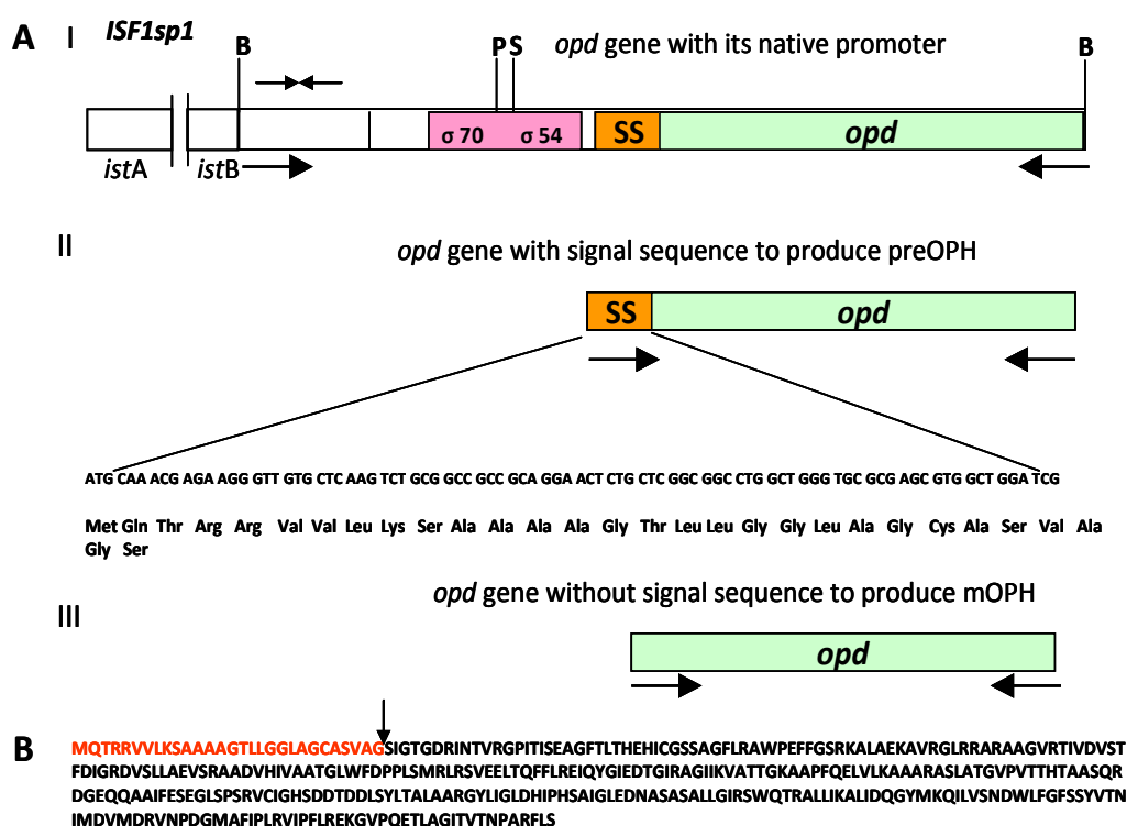
Fig. 5.3. Pane A shows strategies used to clone the opd gene in to P. jinjuensis biotype acephalyticus . Panel B represents amino acid sequence of OPH. Signal peptide sequence was shown in red letters. Signal peptide cleavage site is shown with arrow mark.
