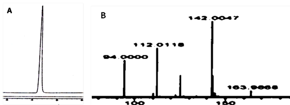
Fig. 4.6. Panel A shows the liquid chromatogram showing single peak of methamidophos with retention time 4.2 min. Panel B shows mass spectrum of methamidophos showing molecular mass as 142.
