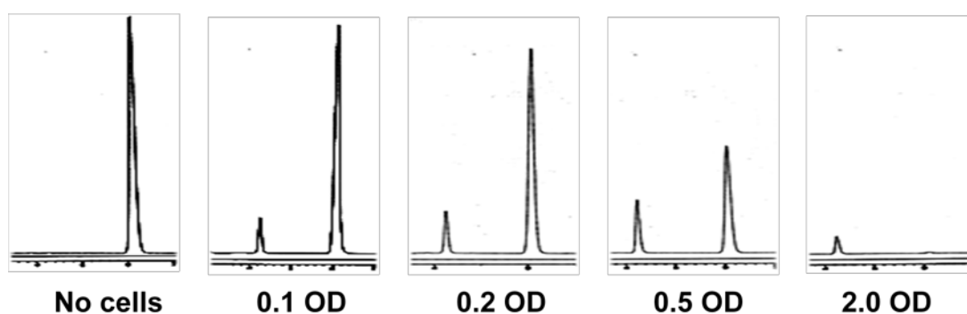
Fig. 4.7. Cell density dependent degradation of acephate. Formation of methamidophos is seen at retention time 4.3 min within 15 min of incubation at 30°C. Progressive disappearance of acephate is seen in liquid chromatograms obtained from the reaction mixtures incubated with different cell densities. Similar pattern is obtained with increase in incubation time.
