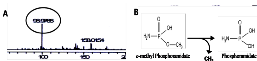
Fig. 4.10. Panel A shows the mass spectrum of phosphoramidate showing the molecular mass 98.9. The phosphoramidate peak appeared at retention time of 2.7 min. Panel B shows chemical reaction indicating formation of phosphoramidate from o -methyl phosphoramidate through dealkylation reaction.
