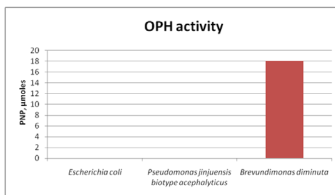
Fig. 5.2. OPH activity in cell lysates of E.coli , P.jinjuensis biotype acephalyticus and Brevundimonas diminuta . OPH activity is expressed as \mu moles of PNP produced per minute/mg of protein.
