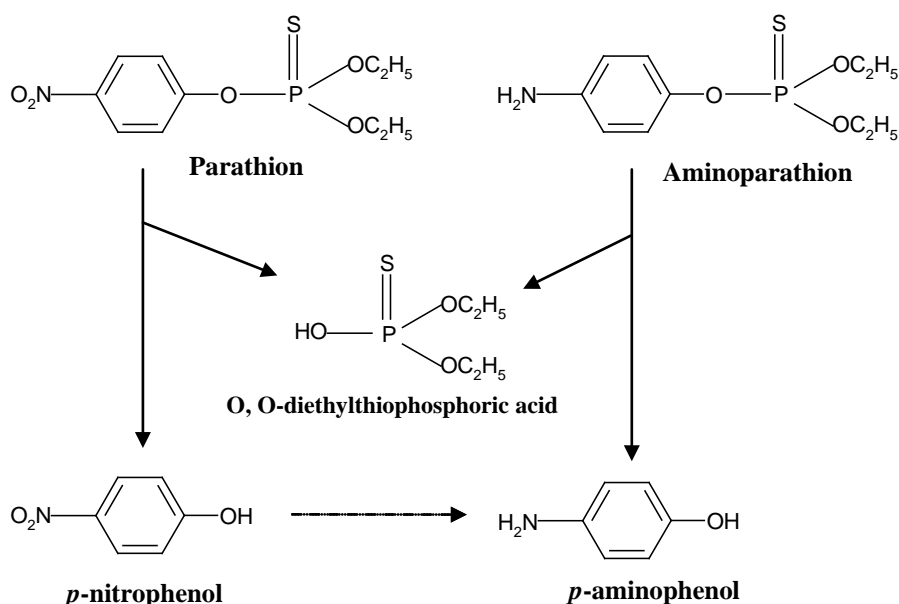
Fig.1.5. Proposed pathway of parathion degradation in flooded soils by Flavobacterium sp. (Adhya et al, 1981).
