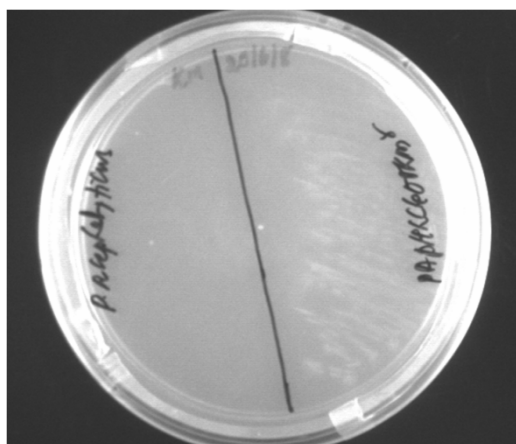
Fig. 5.8. Growth of exconjugants on acephate kanamycin plate. The wild type cells, sensitive to kanamycin failed to grow on acephate kanamycin plates.
