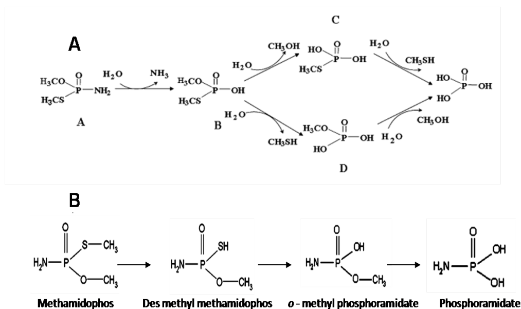
Fig. 4.13. Degradation of methamidophos as reported in Hyphomicrobium species MAP-1 (Panel A) and in P.jinjuensis biotype acephalyticus (Panel B).
