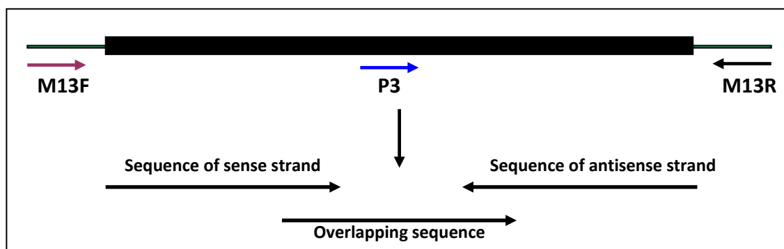
Fig. 3.9 Strategy used for obtaining complete sequence of 16S rRNA gene of strain DS004. Filled bar indicates 16S rRNA gene. Vector sequences corresponding to the M13 forward and reverse primer binding sites are shown with thick lines. Sequence obtained using various primers are shown with thick arrows.
