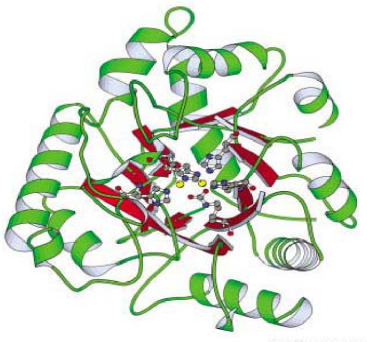
Fig.1.9. Ribbon diagram for the structure of the bacterial phosphotriesterase (Bening et al., 2001).
