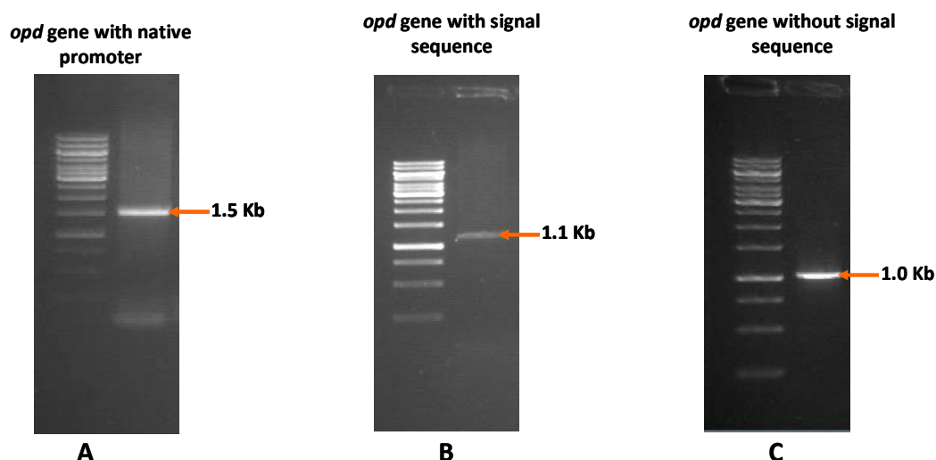
Fig. 5.9. Colony PCR showing the existence and stable maintenance of expression plasmids pMMBKMOPD, pHLCKMOPD and pHNSKMOPD in P.jinjuensis biotype acephalyticus . In Panel A Lane 1 kb ladder, lanes 2 represent exconjugants of P.jinjuensis biotype acephalyticus containing pMMBKMOPD. Panel B, Lane 1 kb ladder, lane 2 represent exconjugants containing expression plasmid pHLCKMOPD. Panel C, Lane 1 kb ladder, lane 2 represents exconjugants containing expression plasmid pHNSKMOPD.
