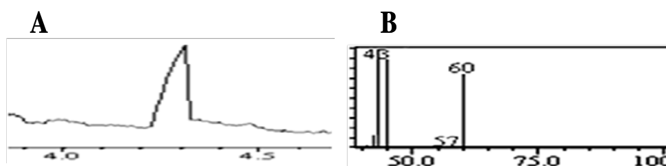
Fig. 4.3. Panel A shows gas chromatogram showing a single peak of acetic acid with retention time 4.3 min. Panel B shows mass spectrum of acetic acid showing the presence of acetic acid with molecular mass 60.
