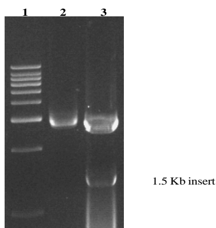
Fig. 3.7 Colony PCR for identification of clones with recombinant plasmid.
