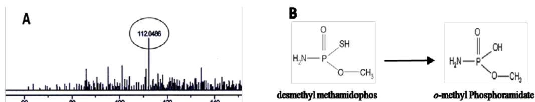
Fig. 4.9. Panel A shows the mass spectrum of o -methyl phosphoramidate showing the molecular mass 112. The peak in chromatogram appeared at 2.62 min. Panel B shows the chemical reaction indicating the formation of o -methyl phosphoramidate from desmethyl methamidophos through oxidation reaction.
