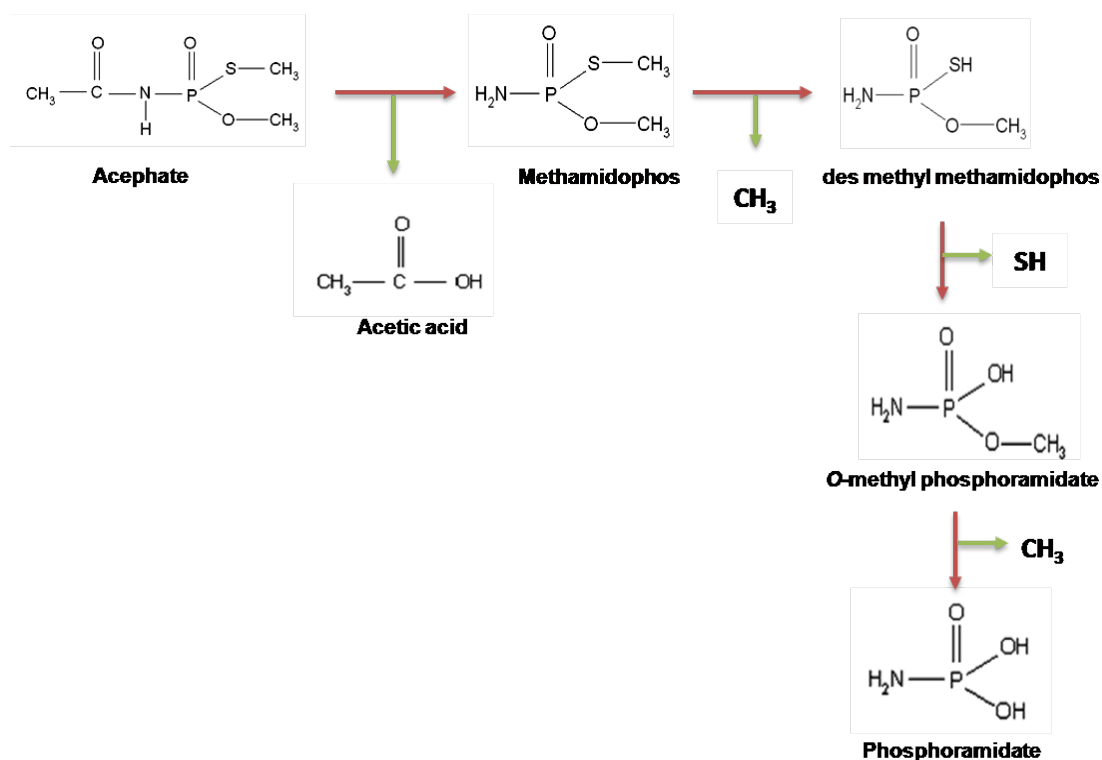
Fig. 4.11. Putative acephate degradation pathway in Pseudomonas jinjuensis biotype acephalyticus .
