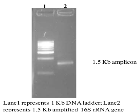
Fig. 3.6. Amplification of 16S rRNA gene from strain DS004.
