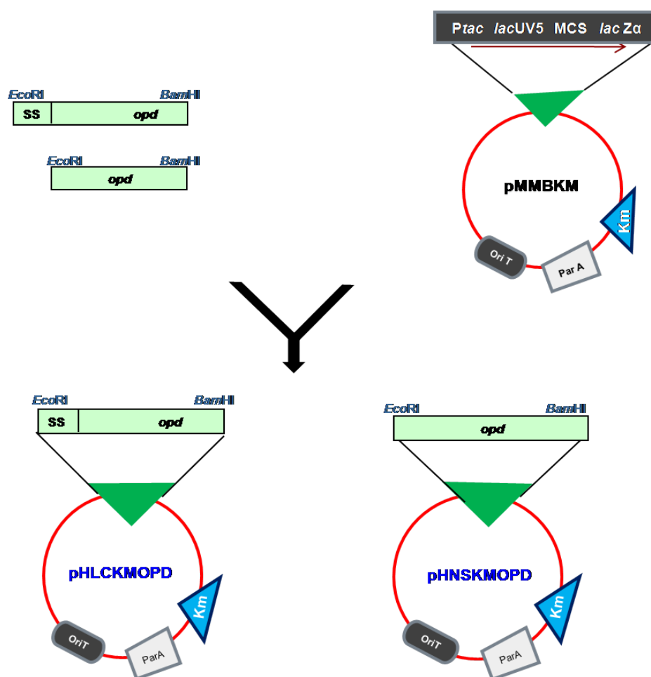
Fig. 5.6. Strategy used for construction of expression plasmids coding precursor (preOPH) and mature (mOPH) forms of OPH with C-terminal his-tags.
