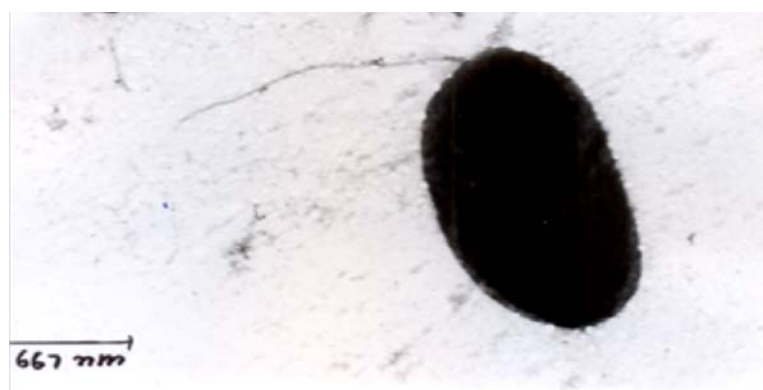
Fig. 3.41 C Transmission electron micrograph of strain DS004.
