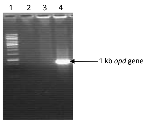
Fig. 5.1. Lane 1 represents 1 Kb DNA ladder; lane 2, 3 and 4 represents PCR reaction mix containing genomic DNA of E.coli , Pseudomonas jinjuensis biotype acephalyticus and Brevundimonas diminuta . Amplification of 1.0 Kb opd gene is shown with arrow mark.
