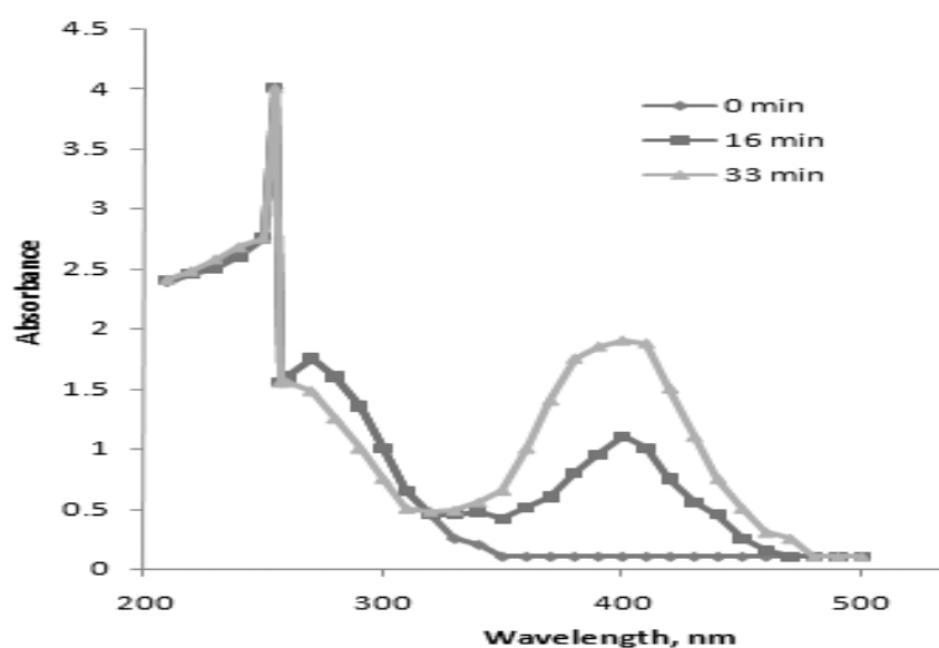
Fig. 5.17. Degradation of Paraoxon by Pseudomonas jinjuensis biotype acephalyticus expressing mOPH.
