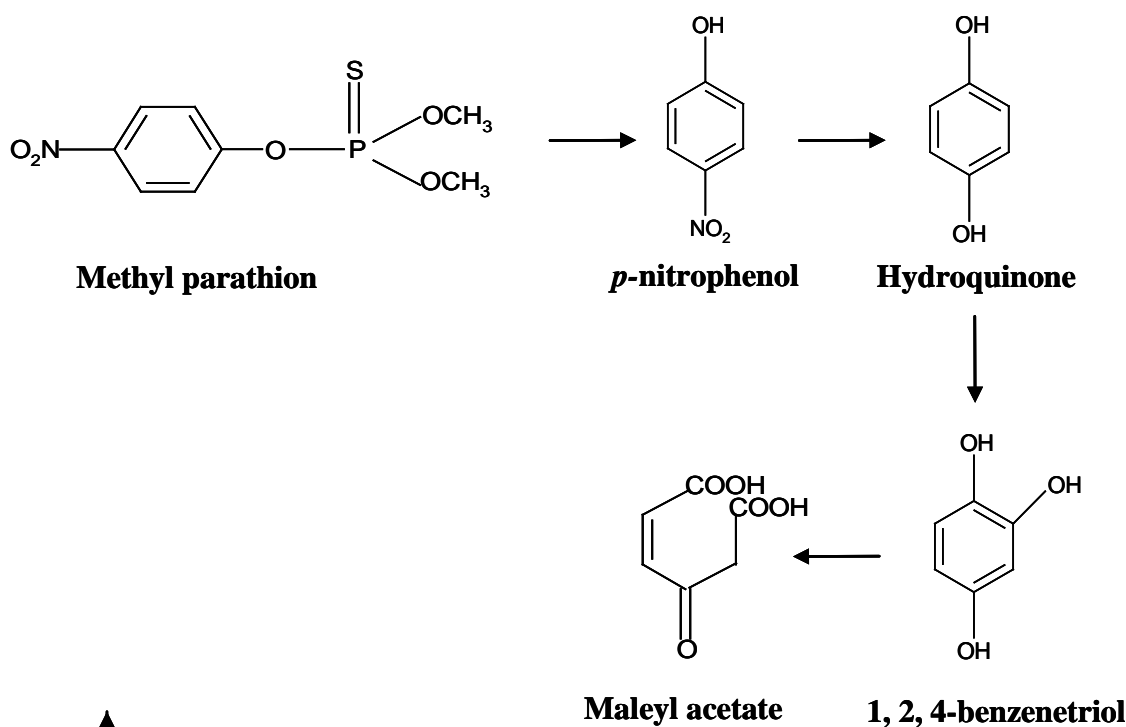
Fig.1.8. Proposed pathway of methyl parathion degradation by Pseudomonas putida (Rani and Lalithakumari, 1994).
