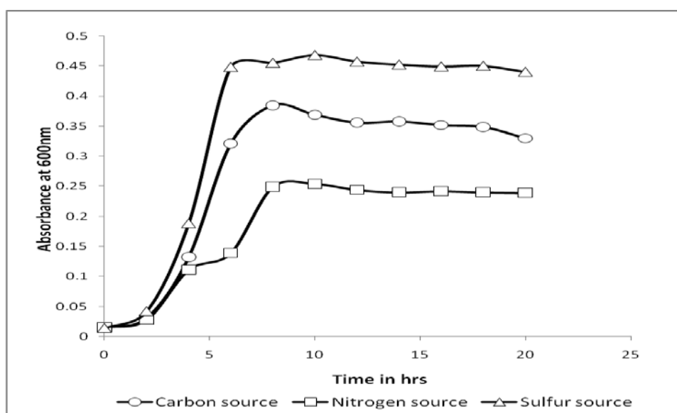
Fig. 3.3 Growth curves of strain DS004 by utilizing acephate as carbon, nitrogen and sulfur source.
