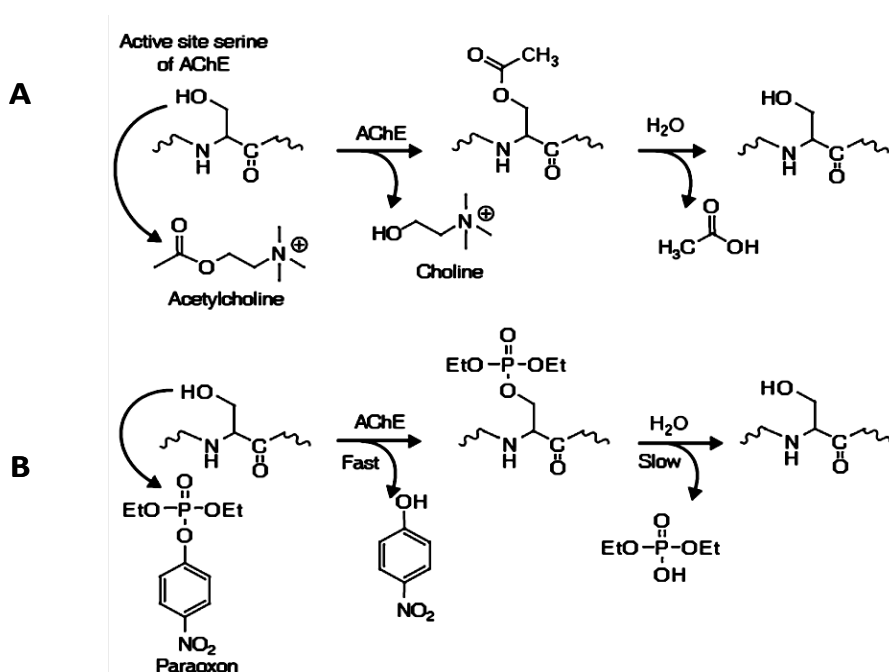
Fig.1.4. Panel A. Acetylcholinesterase (AChE) mediated hydrolysis of acetylcholine. Panel B. Mechanism of inhibition of acetylcholinesterase (AChE) by organophosphates.
