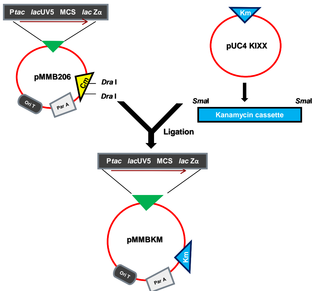
Fig. 5.4. Construction of expression vector pMMBKM.
