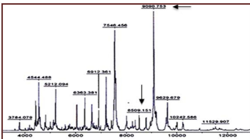
Fig. 3.5 A Mass spectrum showing the E.coli genus specific peak in reference strain E.coli ATCC1775.
