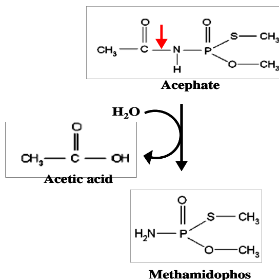
Fig. 4.4 Hydrolysis of acephate to methamidophos and acetic acid by P.jinjuensis biotype acephalyticus .
