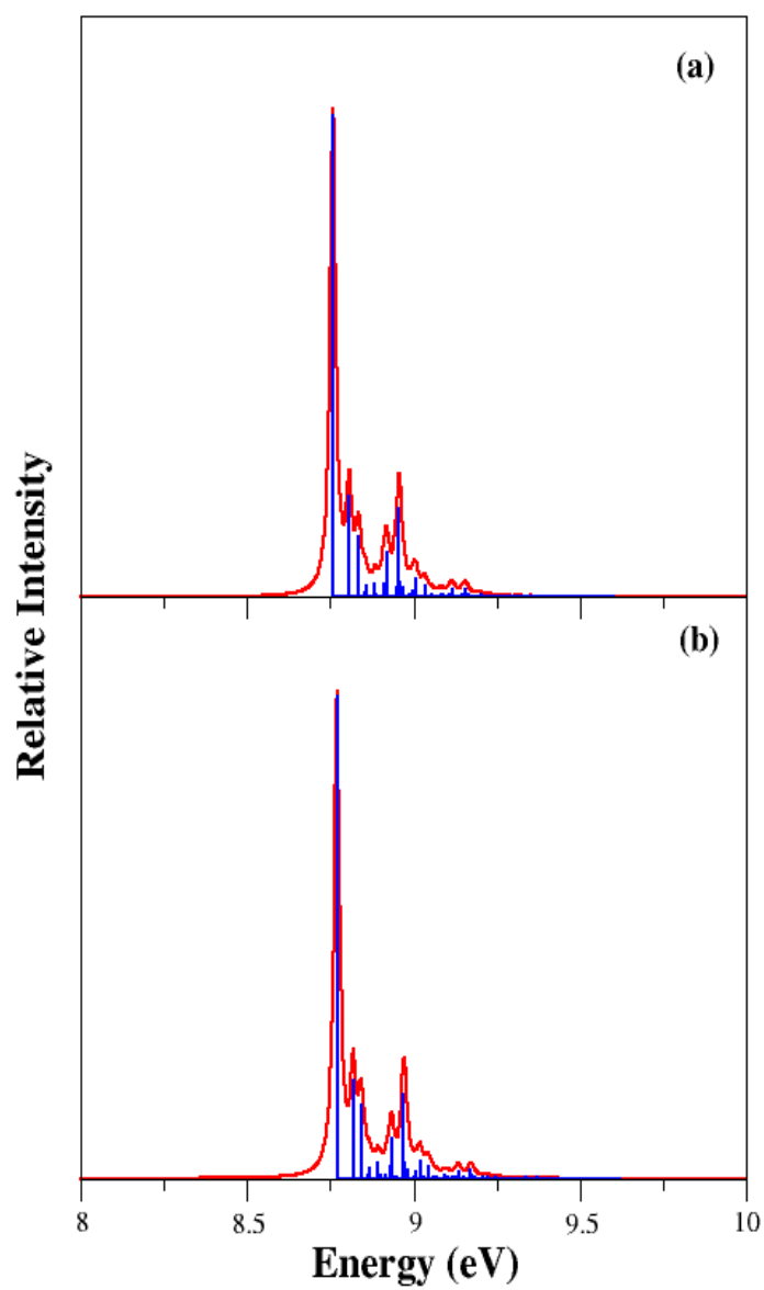
Figure 4.10: Same as in Figure. 4.8 shown for the uncoupled vibronic band of \tilde{B} state of \text{An}^+ .
