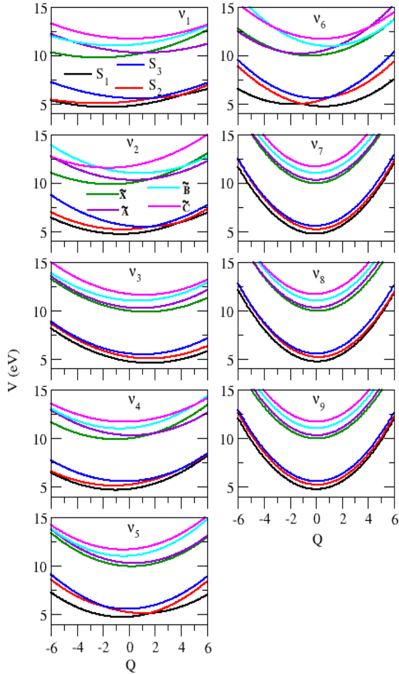
Figure 6.4: Adiabatic potential energies of the \tilde{X} , \tilde{A} , \tilde{B} and \tilde{C} for electronic states of Pym + and S_1 , S_2 and S_3 electronic states of Pym as a function of the dimensionless normal coordinates of the totally symmetric ( a_1 ) vibrational modes, \nu_1 - \nu_9 by different color line.
