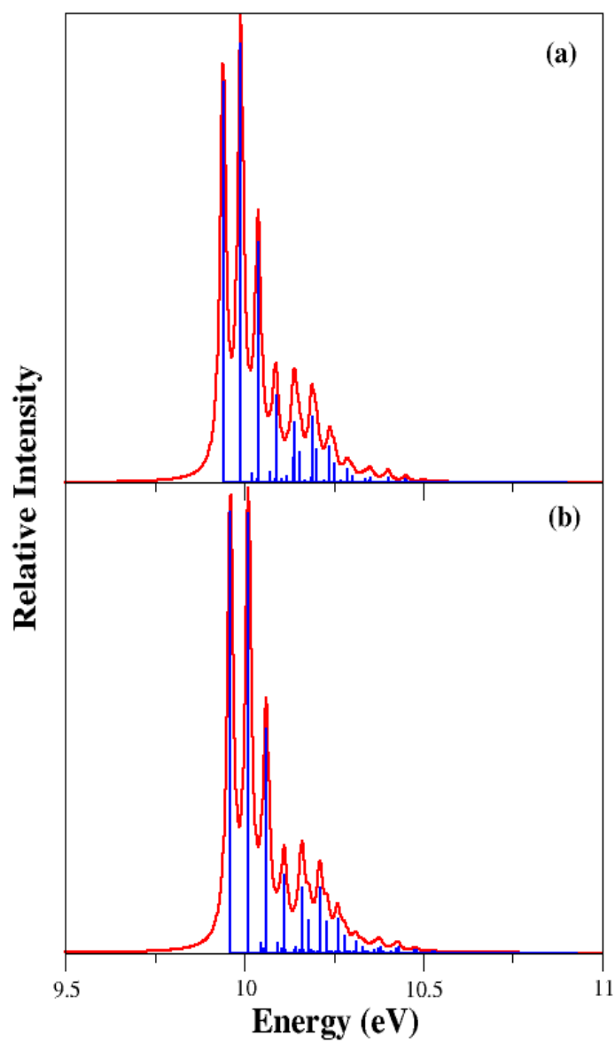
Figure 4.11: Same as in Figure. 4.8 shown for the uncoupled vibronic band of \tilde{C} state of \text{An}^+ .
