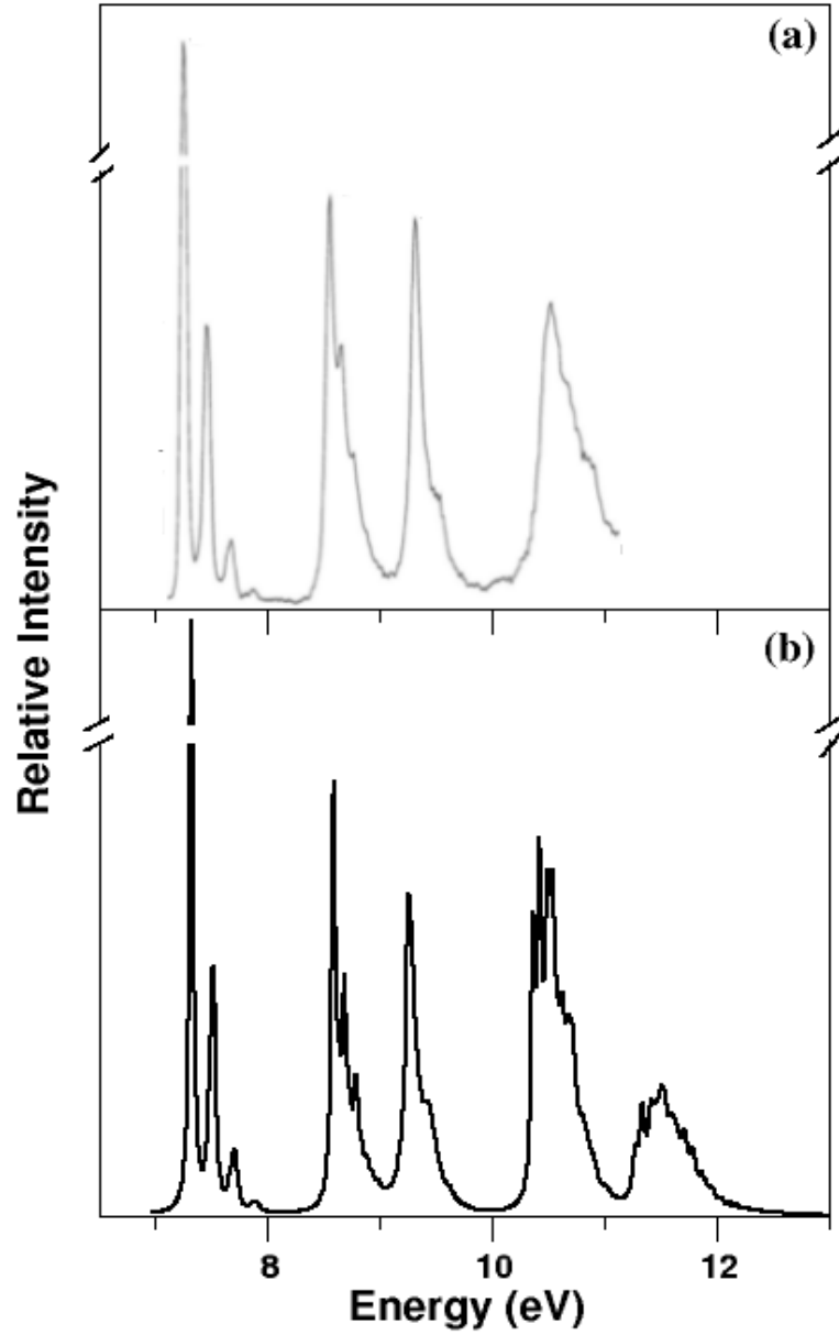
Figure 4.14: The vibronic band structure of the coupled \tilde{X} - \tilde{A} - \tilde{B} - \tilde{C} - \tilde{D} electronic states of \text{An}^+ . The experimental (reproduced from Ref [86]) and the present theoretical results are shown in the top and bottom panels, respectively. The intensity (in arbitrary units) is plotted along the energy (measured relative to electronic ground state ( ^1A_g ) of \text{An} ) of the final vibronic states.
