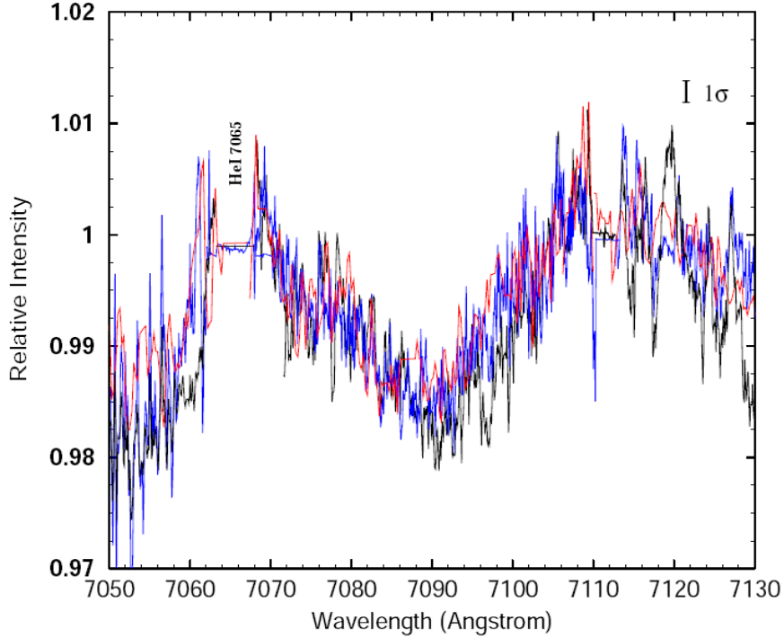
Figure 4.3: The HET and WHT spectra of Cernis 52 corrected for the photospheric and DIB contributions of \text{An}^+ reproduced from Ref. [77].
