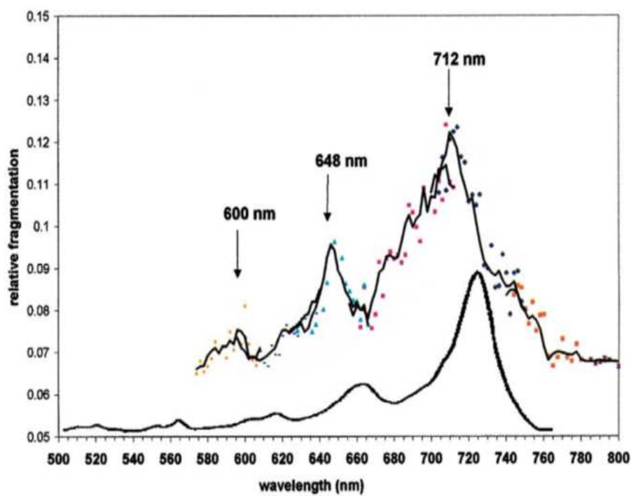
Figure 4.2: The vibrational progression of the D_2 (\tilde{B}) \leftarrow D_0 (\tilde{X}) electronic transition of \text{An}^+ reproduced from Ref. [85].
