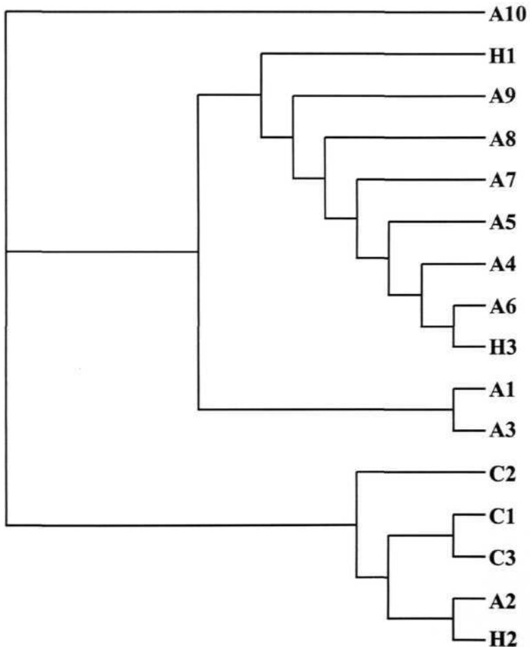
Fig. 16. Dendrogram of sequence polymorphism at a_1 locus in lions
