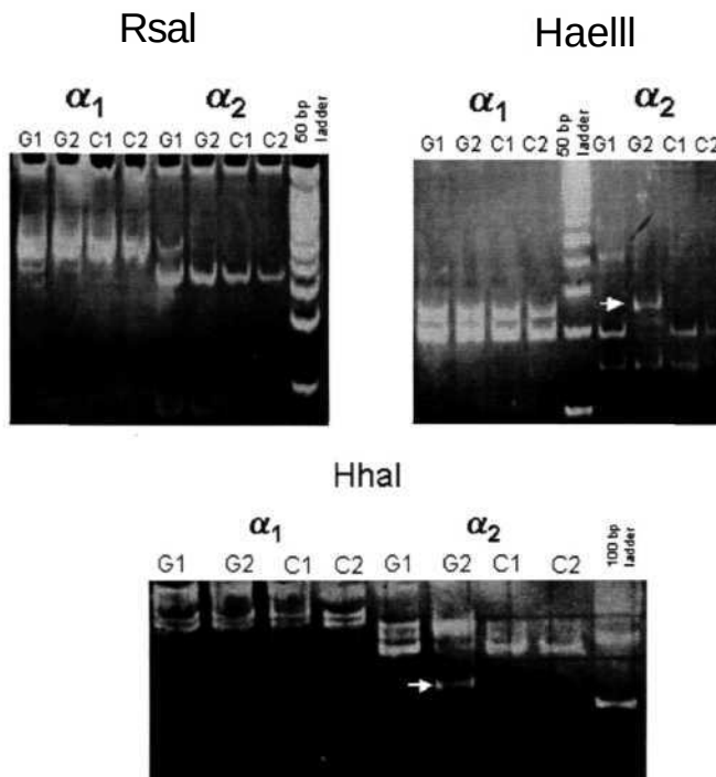
Fig. 10B. PCR Based RFLP (PBR) analysis of \alpha_1 and \alpha_2 locus specific amplicons (Cont'd)
