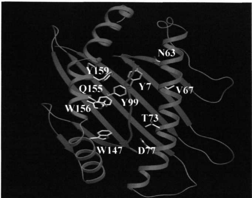
Fig. 46. Amino acid residues in \alpha_1 and \alpha_2 domains of MHC class I involved in binding with foreign peptide
