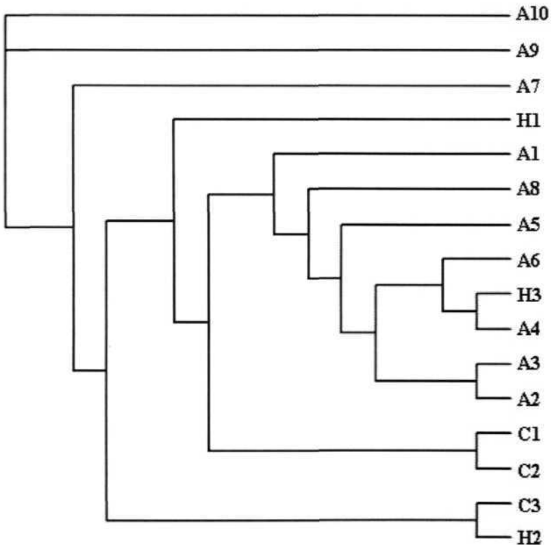
Fig. 20. Dendrogram of sequence polymorphism at a_2 locus in lions
