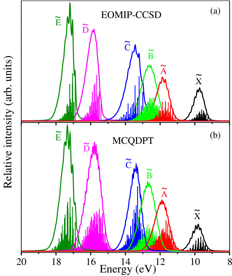
FIGURE 5.5: The photoionization bands of the \tilde{X}^2A' , \tilde{A}^2A' , \tilde{B}^2A'' , \tilde{C}^2A'' , \tilde{D}^2A' , and \tilde{E}^2A' states of the \text{CH}_2\text{NHCH}_2^+ are calculated using the a' vibrational modes and the time-independent matrix diagonalization method (details provided in the text). The relative intensity is plotted as a function of the energy of the vibronic levels.
