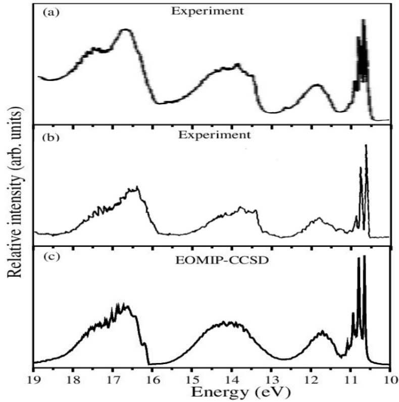
FIGURE 4.5: Vibronic band structure of the coupled \tilde{X}^2B_1 - \tilde{A}^2A_1 - \tilde{B}^2B_2 - \tilde{C}^2A_2 - \tilde{D}^2A_1 - \tilde{E}^2B_1 electronic states of c\text{-C}_2\text{H}_4\text{O}^+ . Relative intensity (in arbitrary units) is plotted as a function of the energy of the vibronic states of c\text{-C}_2\text{H}_4\text{O}^+ . Available experimental spectrum reproduced from Refs. [47] and [86] are shown in panel (a) and (b), respectively. The present theoretical results is shown in panel (c).
