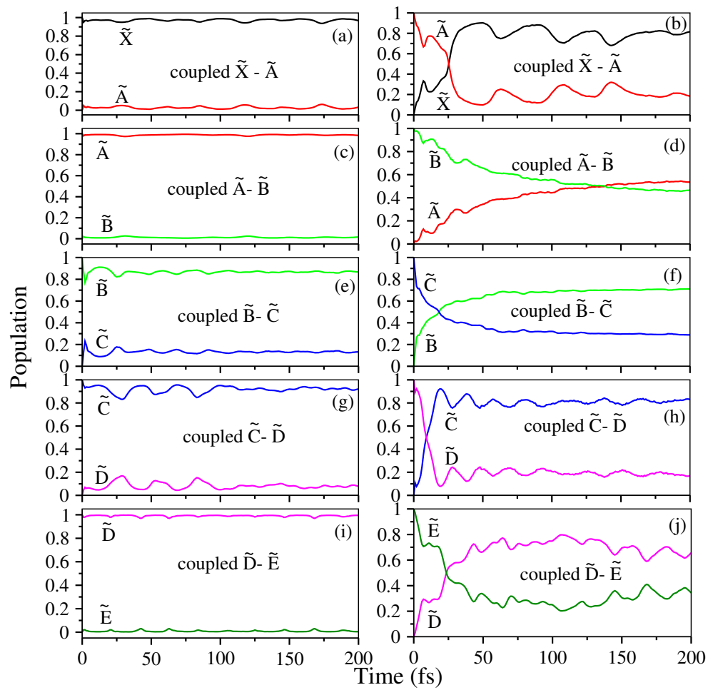
FIGURE B8: Time-dependence of the diabatic electronic populations in the coupled \tilde{X}^2B_1 - \tilde{A}^2A_1 , \tilde{A}^2A_1 - \tilde{B}^2B_2 , \tilde{B}^2B_2 - \tilde{C}^2A_2 , \tilde{C}^2A_2 - \tilde{D}^2A_1 and \tilde{D}^2A_1 - \tilde{E}^2B_1 states dynamics obtained by locating an initial WP on each electronic state separately is shown in the panels (a)–(j), respectively (see text for details).
