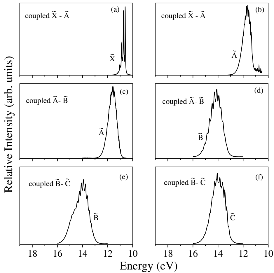
FIGURE B7: Composite vibronic band structure of the coupled \tilde{X}^2\text{B}_1\text{-}\tilde{A}^2\text{A}_1 , \tilde{A}^2\text{A}_1\text{-}\tilde{B}^2\text{B}_2 , \tilde{B}^2\text{B}_2\text{-}\tilde{C}^2\text{A}_2 , \tilde{C}^2\text{A}_2\text{-}\tilde{D}^2\text{A}_1 and \tilde{D}^2\text{A}_1\text{-}\tilde{E}^2\text{B}_1 states of c\text{-C}_2\text{H}_4\text{O}^+ are shown in the panels (a)–(j), respectively.
