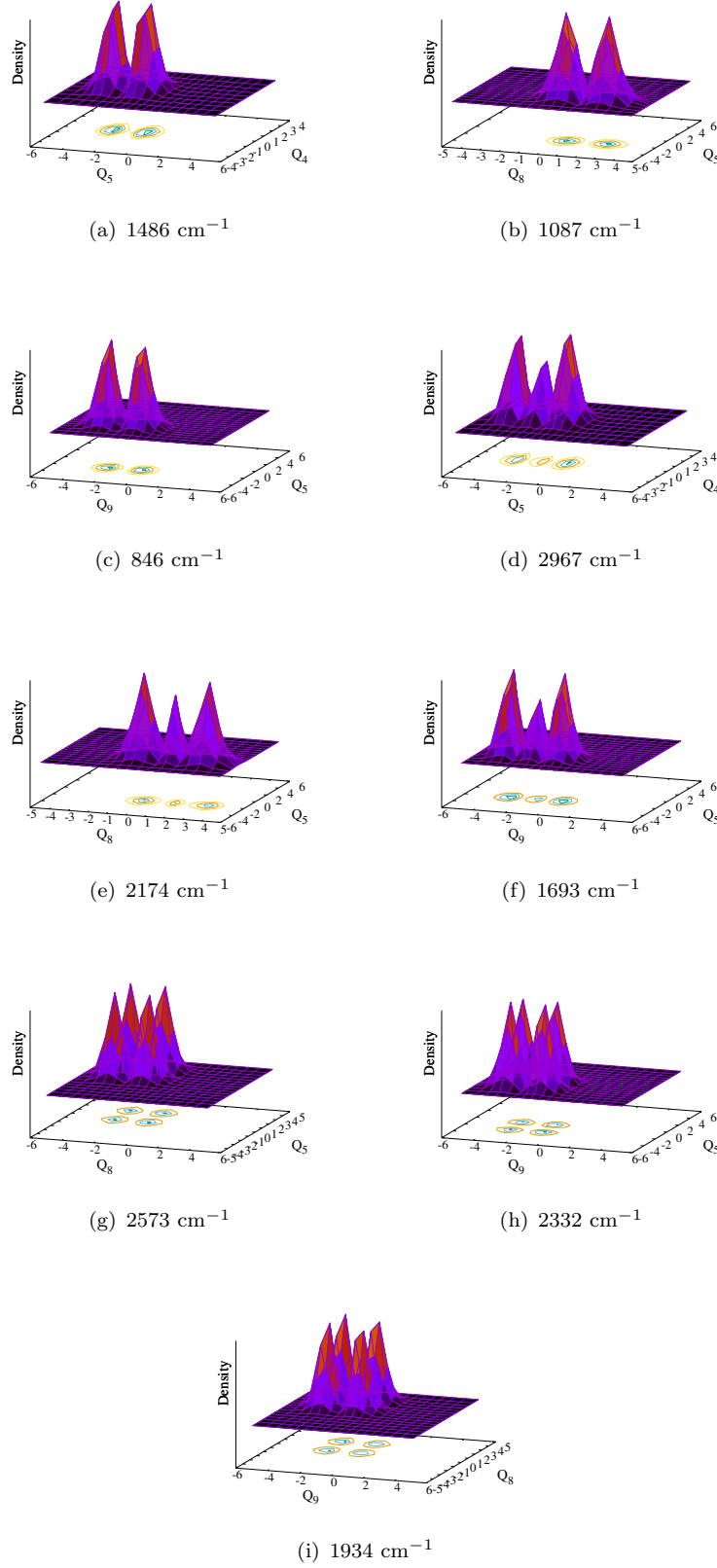
FIGURE A7: Probability density of vibronic wave functions of the \tilde{D}^2A'' electronic state of \text{CH}_3\text{COH}^+ as a function of nuclear coordinate. Panels a, b and c represent the fundamentals \nu_{50}^1 , \nu_{80}^1 and \nu_{90}^1 and panels d, e and f represent the first overtone \nu_{50}^2 , \nu_{80}^2 and \nu_{90}^2 , respectively. The wave functions in panels g, h and i represent the combination peaks \nu_{50}^1 + \nu_{80}^1 , \nu_{50}^1 + \nu_{90}^1 and \nu_{90}^1 + \nu_{80}^1 , respectively.
