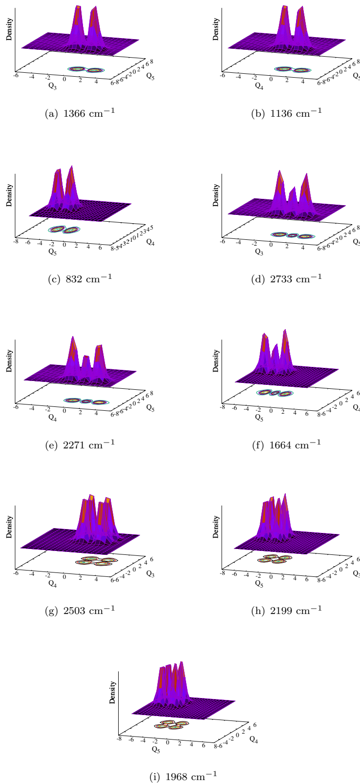
FIGURE B2: Probability density of vibronic wave functions of the \tilde{A}^2A_1 electronic state of c\text{-C}_2\text{H}_4\text{O}^+ as a function of nuclear coordinate. Panels a, b and c represent the fundamental of \nu_{30}^1 , \nu_{40}^1 and \nu_{50}^1 and first overtone of \nu_{30}^2 , \nu_{40}^2 and \nu_{50}^2 modes, the wavefunction in panels g, h and i represent the combination peak of \nu_{40}^1 + \nu_{30}^1 , \nu_{50}^1 + \nu_{30}^1 and \nu_{50}^1 + \nu_{40}^1 .
