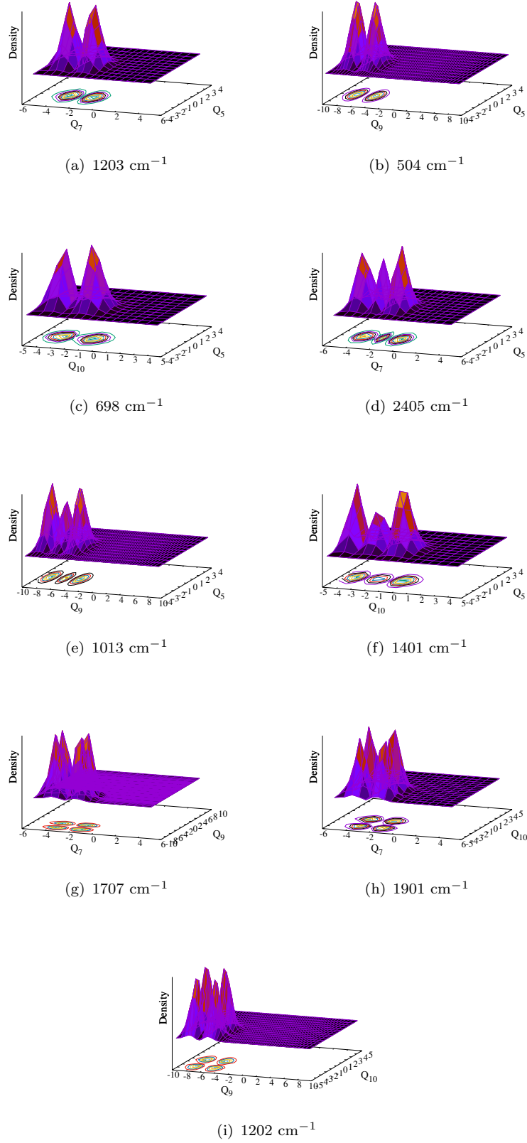
FIGURE C6: Probability density of vibronic wave functions of the \tilde{B} electronic state of \text{CH}_2\text{NHCH}_2^+ with using MCQDPT data as a function of nuclear coordinate. Panels a, b and c represent the fundamental of \nu_{70}^1 , \nu_{90}^1 and \nu_{100}^1 and first overtone of \nu_{70}^2 , \nu_{90}^2 and \nu_{100}^2 modes, the wavefunction in panels g, h and i represent the combination peak of \nu_{70}^1 + \nu_{90}^1 , \nu_{70}^1 + \nu_{100}^1 and \nu_{90}^1 + \nu_{100}^1 .
