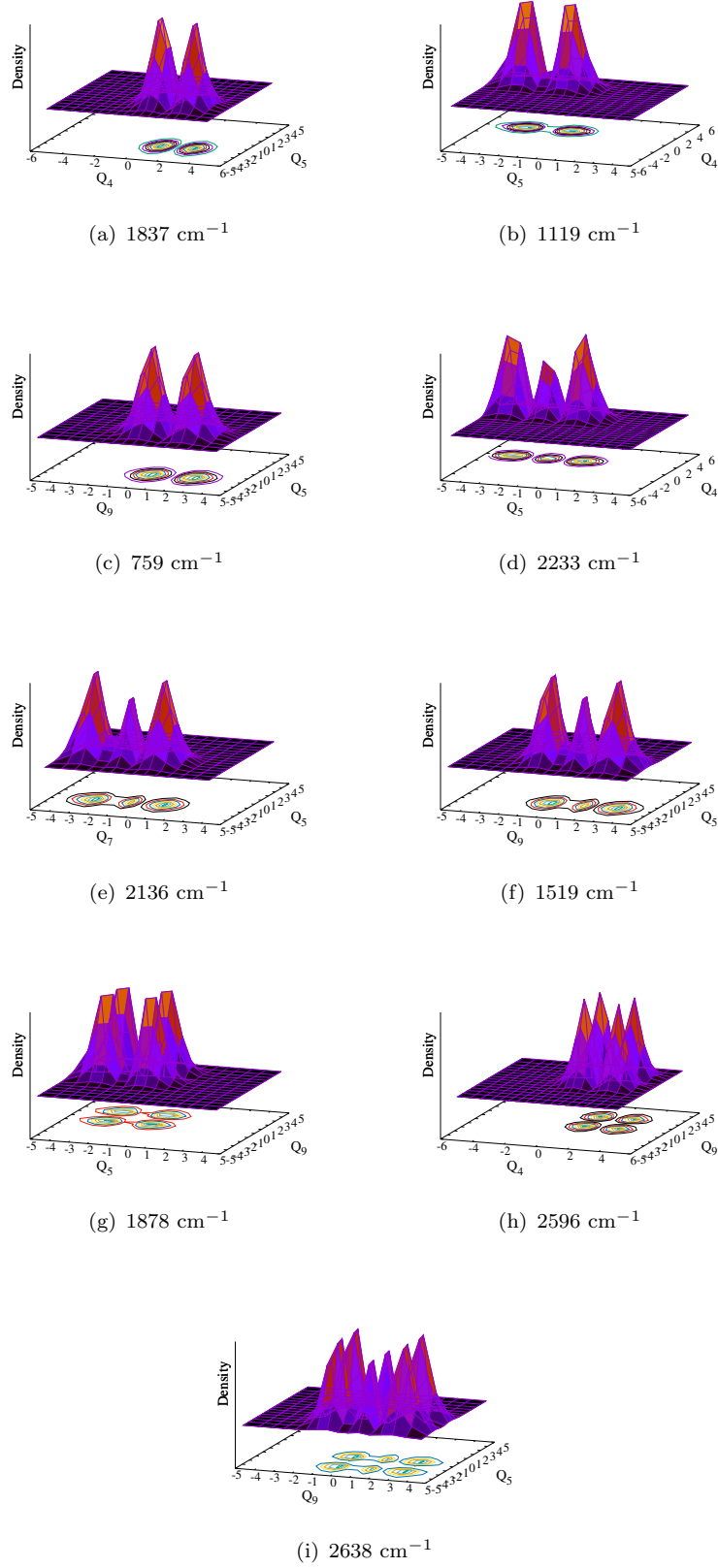
FIGURE A4: Probability density of vibronic wave functions of the \tilde{A}^2A'' electronic state of \text{CH}_3\text{COH}^+ as a function of nuclear coordinate. Panels a, b and c represent the fundamentals \nu_{40}^1 , \nu_{50}^1 and \nu_{90}^1 and panels d, e and f represent the first overtone \nu_{50}^2 , \nu_{70}^2 and \nu_{90}^2 , respectively. The wave functions in panels g, h and i represent the combination peaks \nu_{50}^1 + \nu_{90}^1 , \nu_{40}^1 + \nu_{90}^1 and \nu_{90}^1 + \nu_{50}^1 , respectively.
