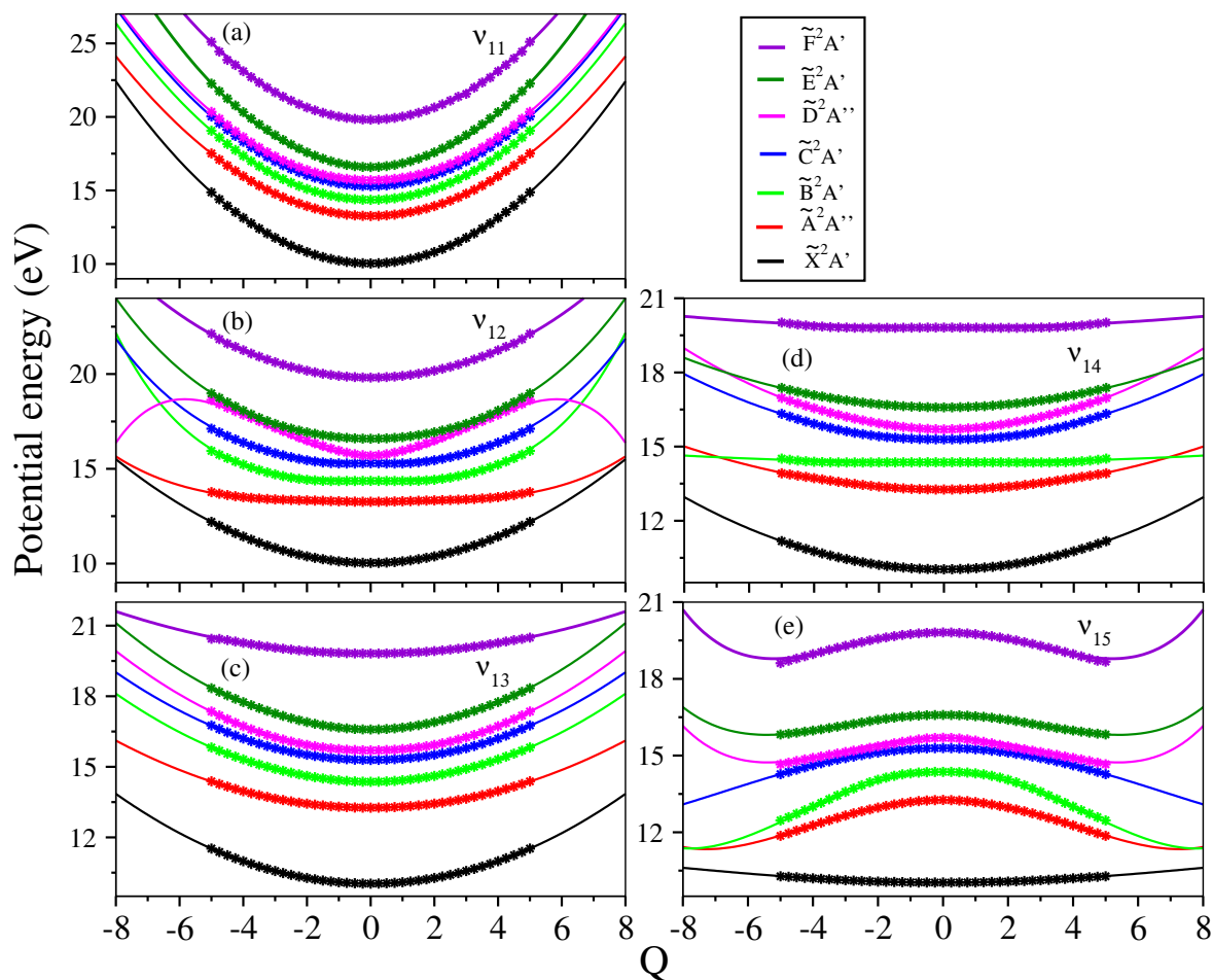
FIGURE A2: The adiabatic PESs of the lowest electronic state \tilde{X}^2A' , \tilde{A}^2A'' , \tilde{B}^2A' , \tilde{C}^2A' , \tilde{D}^2A'' , \tilde{E}^2A' and \tilde{F}^2A' of \text{CH}_3\text{COH}^+ plotted along the normal displacement coordinate of the a'' vibrational modes, \nu_{11} - \nu_{15} . The solid lines are obtained from the theoretical model and the calculated ab initio potential energies are shown by the asterisks.
