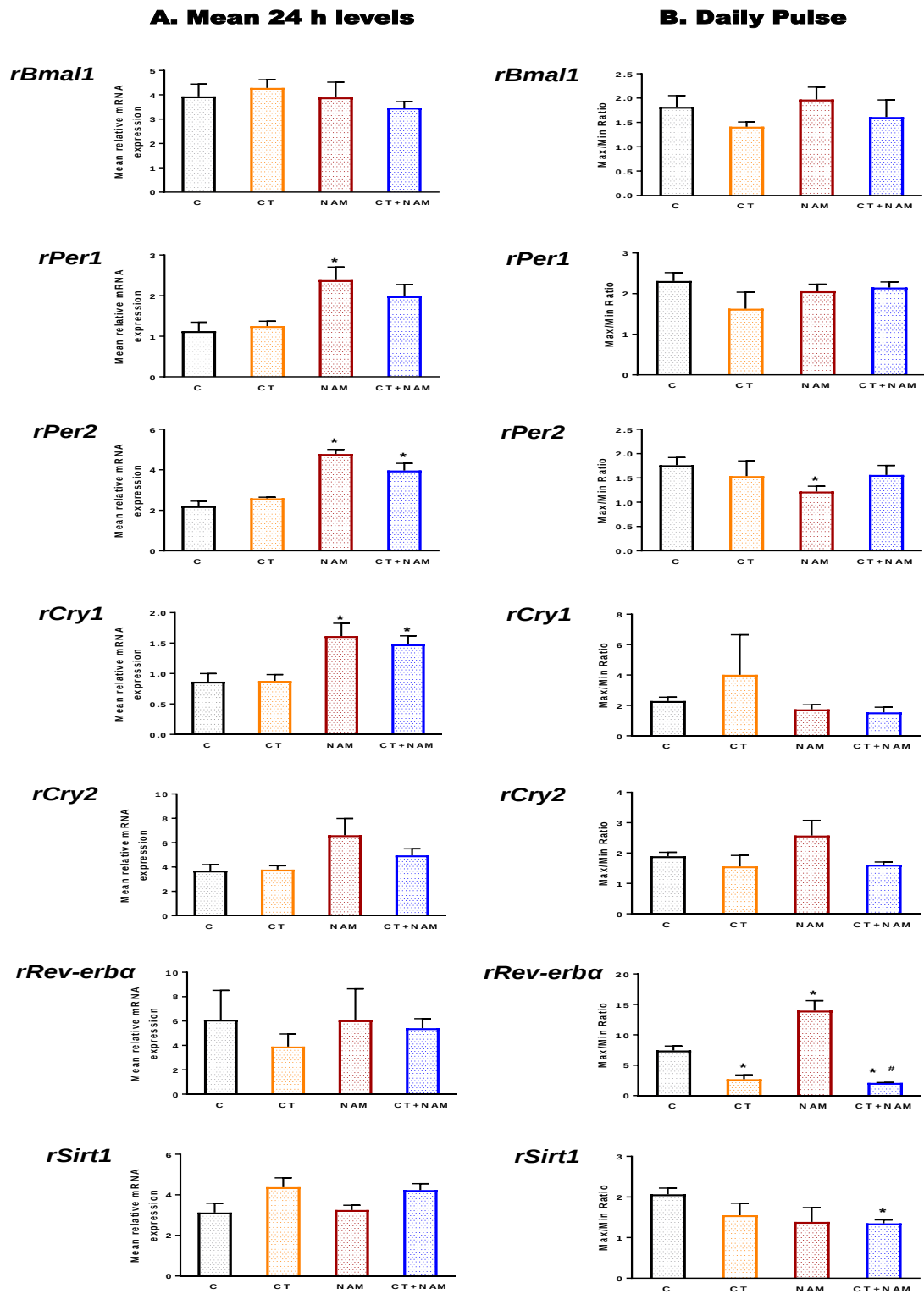
Fig. 39 (A) Mean 24 h levels and (B) daily pulse of rBmal1 , rPer1 , rPer2 , rCry1 , rCry2 , rRev-erba and rSirt1 mRNA in the SCN explants. Each value is mean \pm SEM, p < 0.05 and expressed as mean relative gene expression. ‘*’ Indicates statistically significant difference ( p < 0.05 ). C – control; CT – curcumin treated; NAM – nicotinamide treated; CT+NAM – co-treated with curcumin and nicotinamide.
