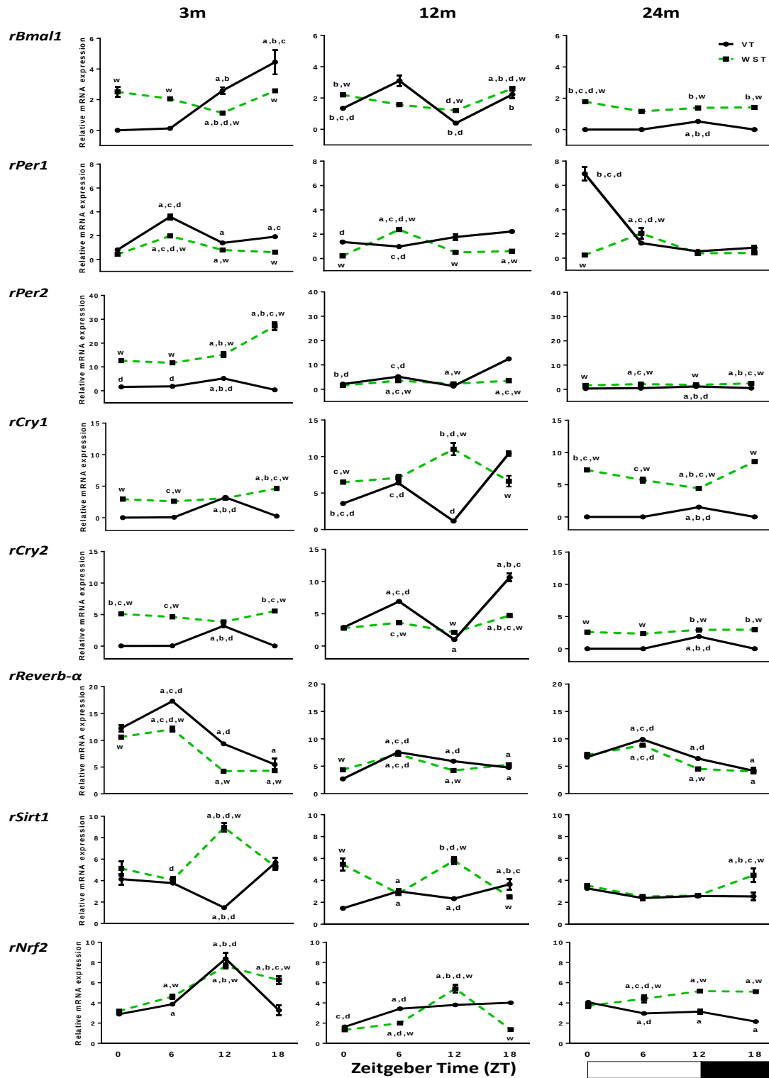
Fig. 32 Effect of W. somnifera treatment on daily rhythms of clock genes, rSirt1 and rNrf2 mRNA expression in the aging rat SCN in 3, 12 and 24 months (m). Each value is mean \pm SEM (n = 4), p < 0.05 and expressed as relative gene expression. p_a < 0.05 ; p_b < 0.05 , p_c < 0.05 and p_d < 0.05 (where 'a', 'b', 'c' and 'd' refers to comparison with ZT-0, ZT-6, ZT-12 and ZT-18 respectively within the group). p_w < 0.05 (where 'w' refers to comparison of gene expression levels at same time point in the age matched vehicle group).
