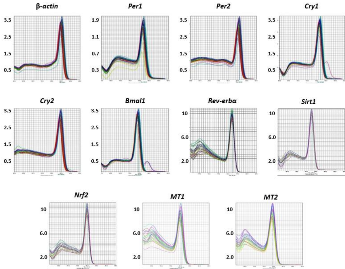
Fig. 24 Representative Dissociation curves showing specific amplification of target genes
