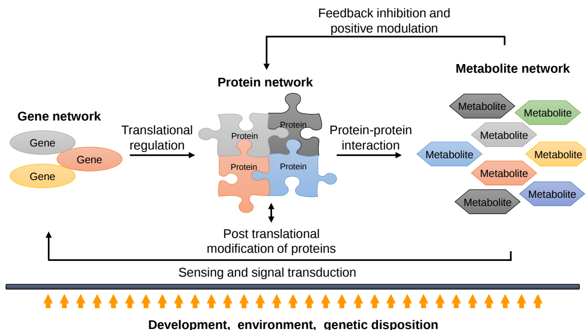
Fig. 10 Diagrammatic representation of the gene-protein-metabolite network (Weckwerth 2003).
