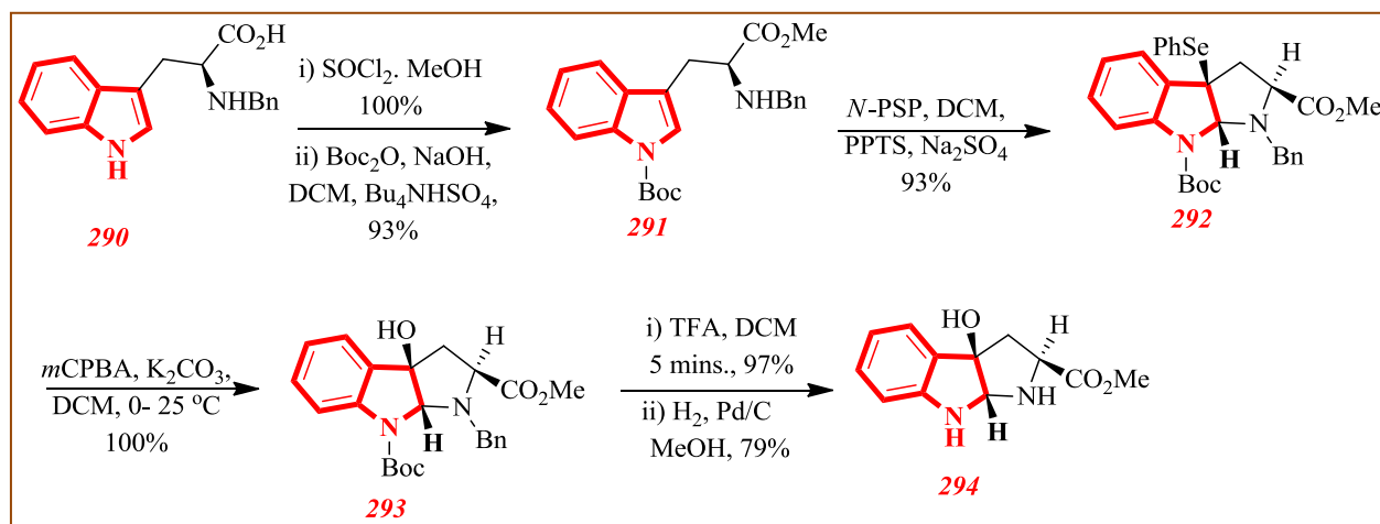
Eqn. 48: Stereocontrolled synthesis of 3 \alpha -hydroxy-pyrroloindole
