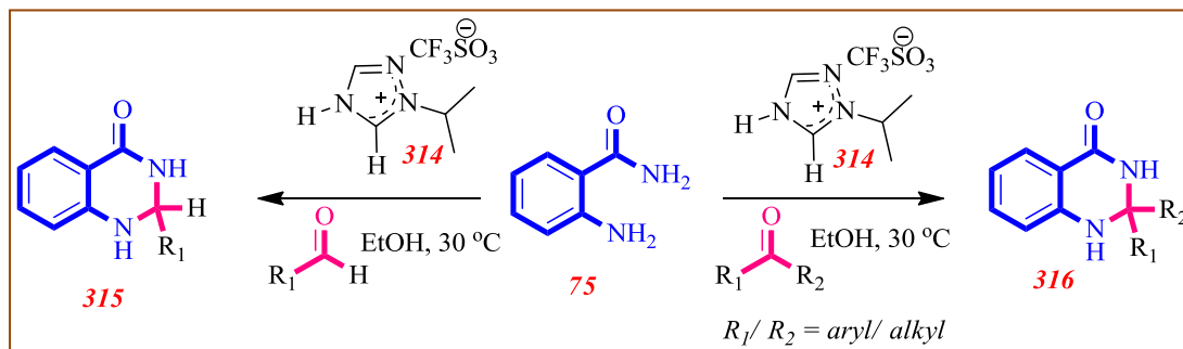
Eqn. 56. Synthesis of quinazolinones via ionic liquid catalyst
