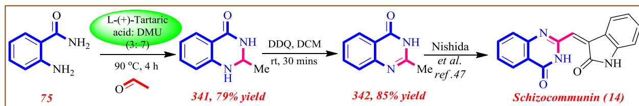
Scheme 13. Formal Synthesis of Schizocommunin
