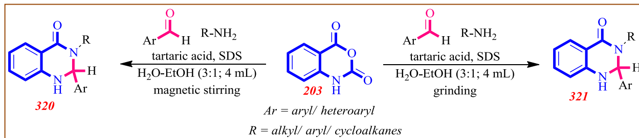
Eqn. 58. Synthesis of quinazolinones via natural acid/ SDS catalysis
