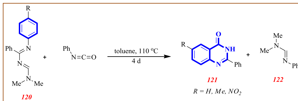
Eqn. 11. Synthesis of 2-substituted-quinazolinones via hetero Diels-Alder reaction
