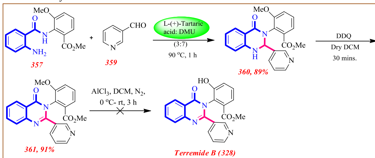
Scheme 20: Synthesis of Terremide B
