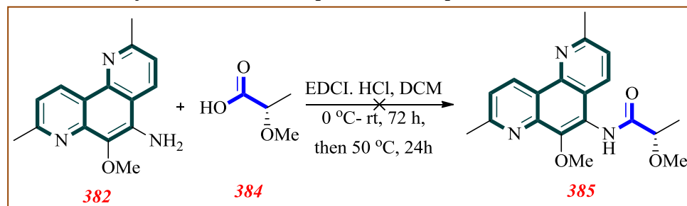
Scheme 24. Synthesis of enantiospecific Actinophenanthroline A
