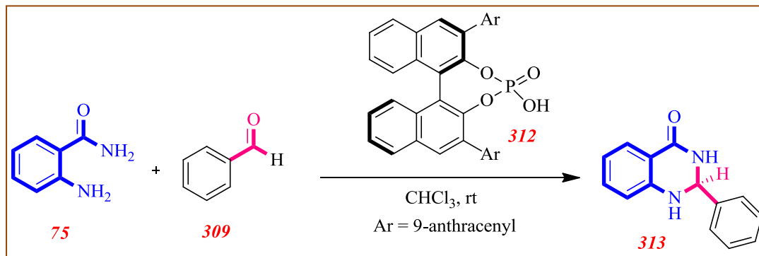
Eqn. 55. Synthesis of quinazolinones via asymmetric Brønsted acid catalyst
