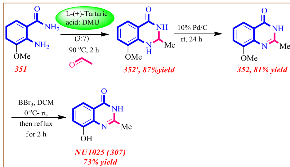
Scheme 17: Synthesis of 8-hydroxy-2-methylquinazolin-4(3 H )-one ( NU1025 )
