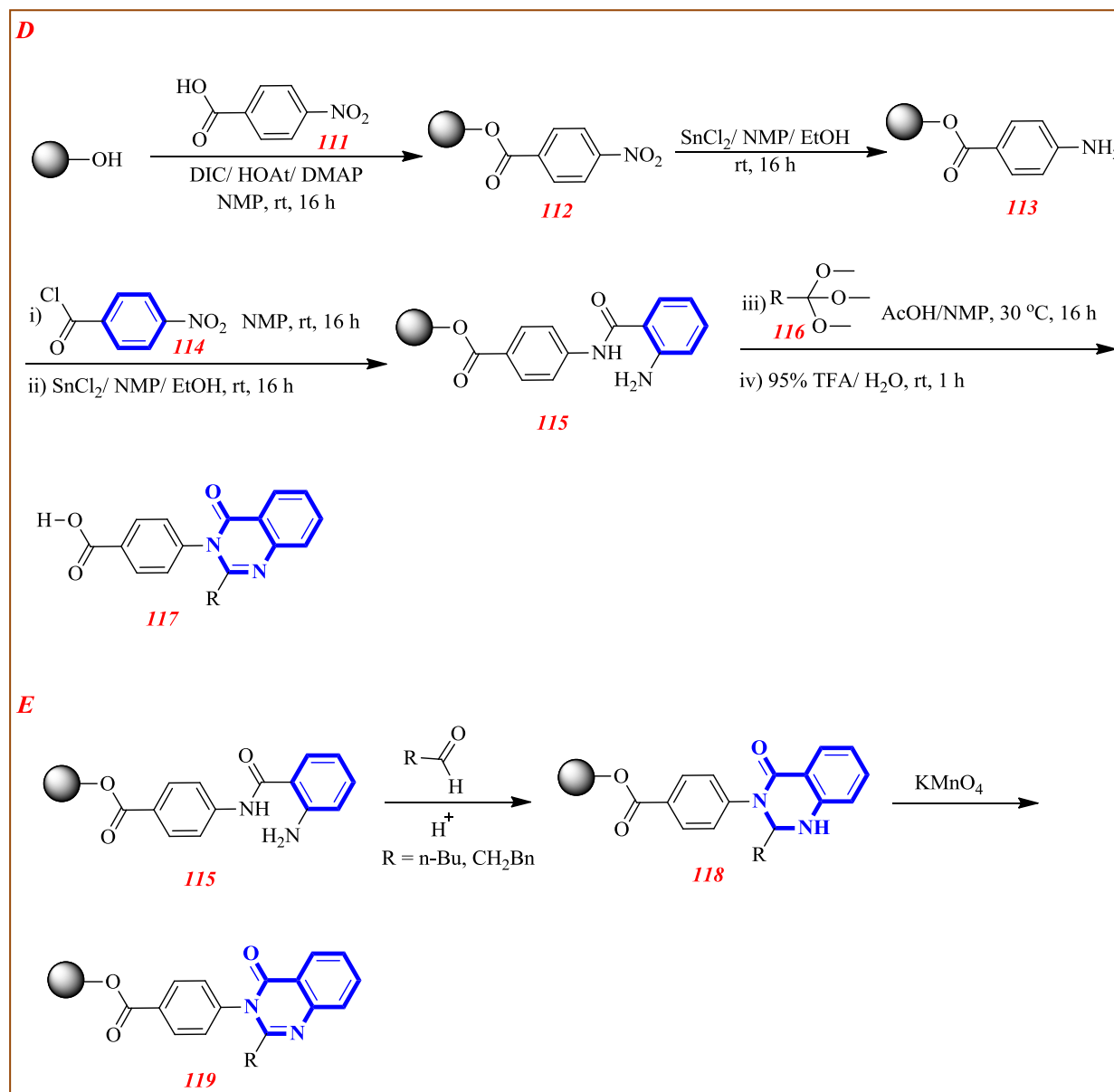
Eqn. 10. Synthesis of various quinazolinones via solid phase
