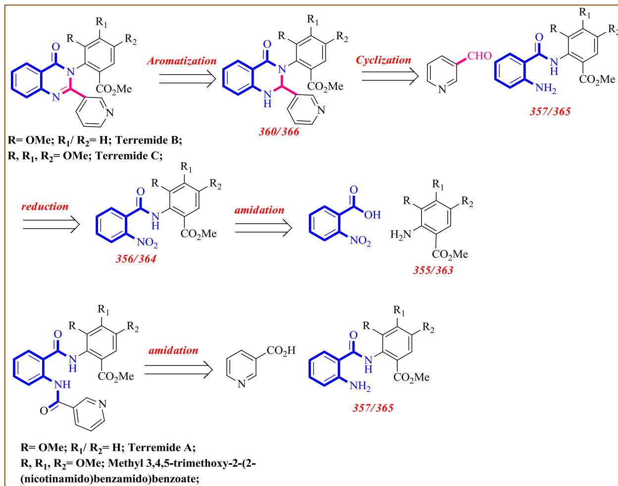
Scheme 18: Retrosynthesis of Terremide A, B, C and Methyl 3,4,5-trimethoxy-2-(2-(nicotinamido)benzamido)benzoate
