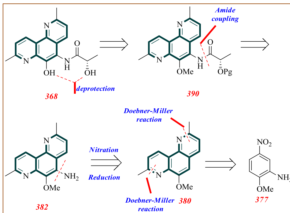
Scheme 22. Retrosynthetic analysis
