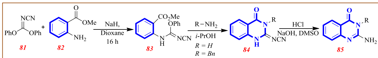
Eqn. 5. Condensation between methyl anthranilate with carbonimides
