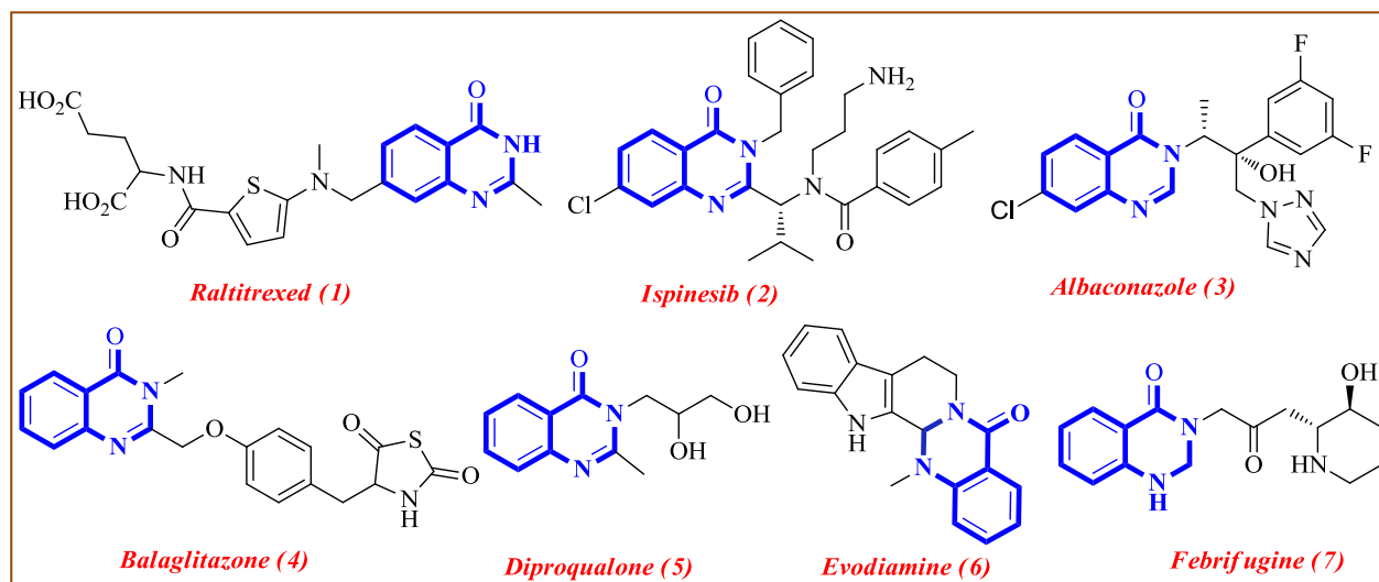
Figure 3. Representation of some important quinazolinone drugs
