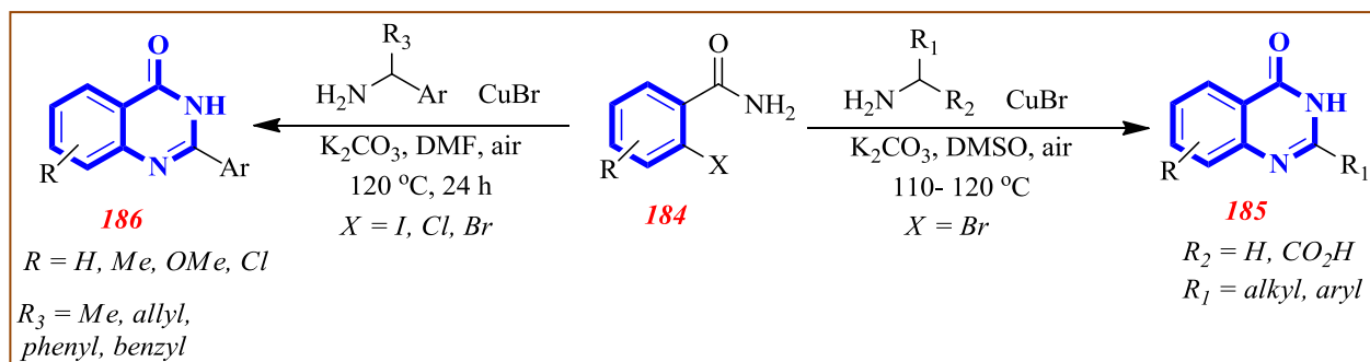
Eqn. 22. Cu catalyzed benzylamine cyclization
