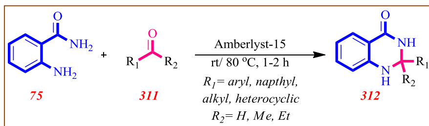
Eqn. 54. Synthesis of quinazolinones via heterogeneous solid acid catalyst
