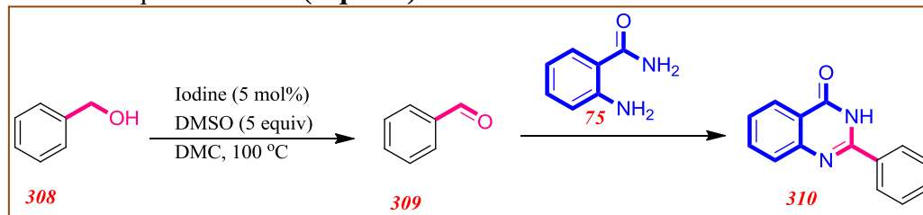
Eqn. 53. Iodine catalyzed synthesis of quinazolinones
