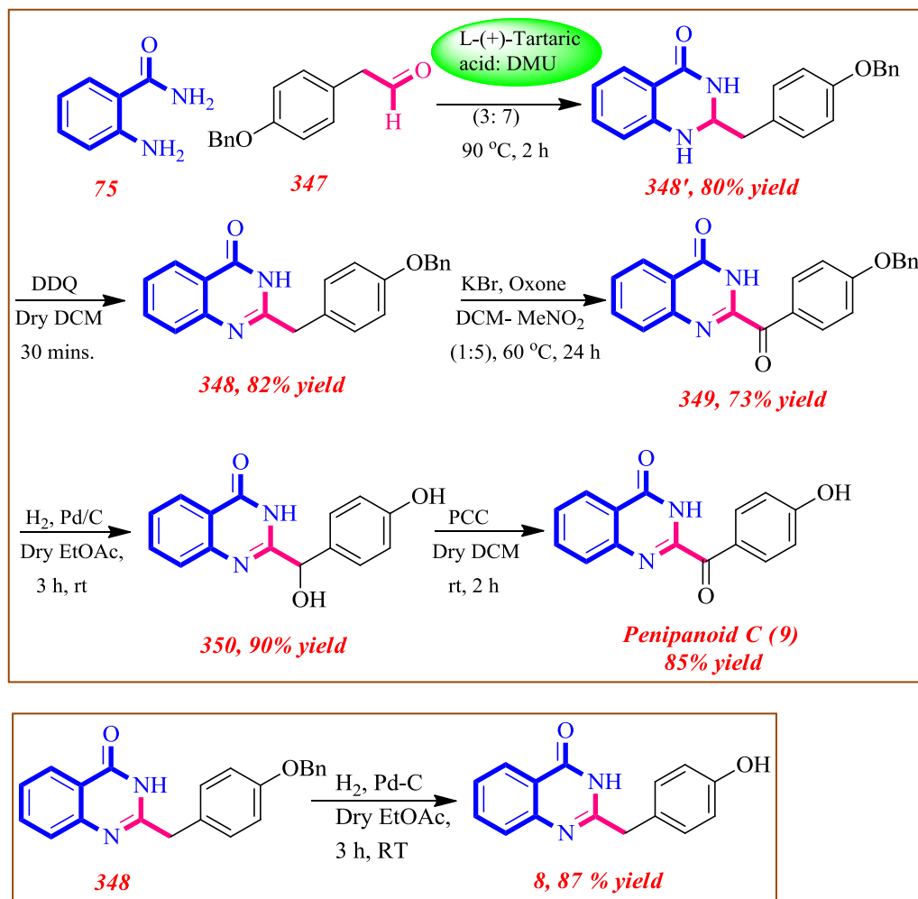
Scheme 16: Revised synthesis of 2-(4-hydroxybenzyl)quinazolin-4(3H)-one and penipanoid C
