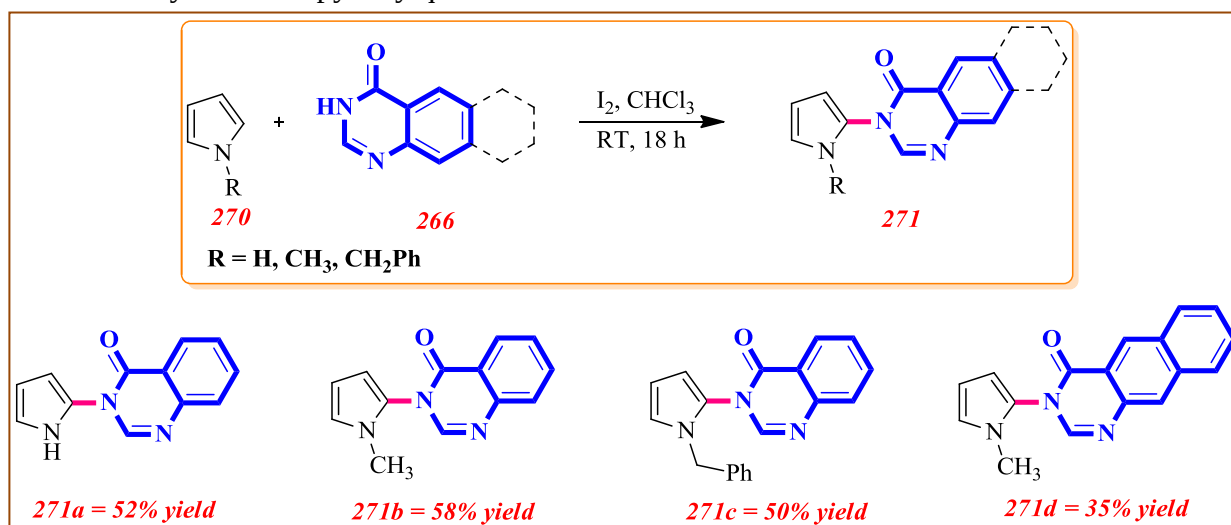
Scheme 3: Synthesis of pyrrolylquinazolinone derivatives [a]
