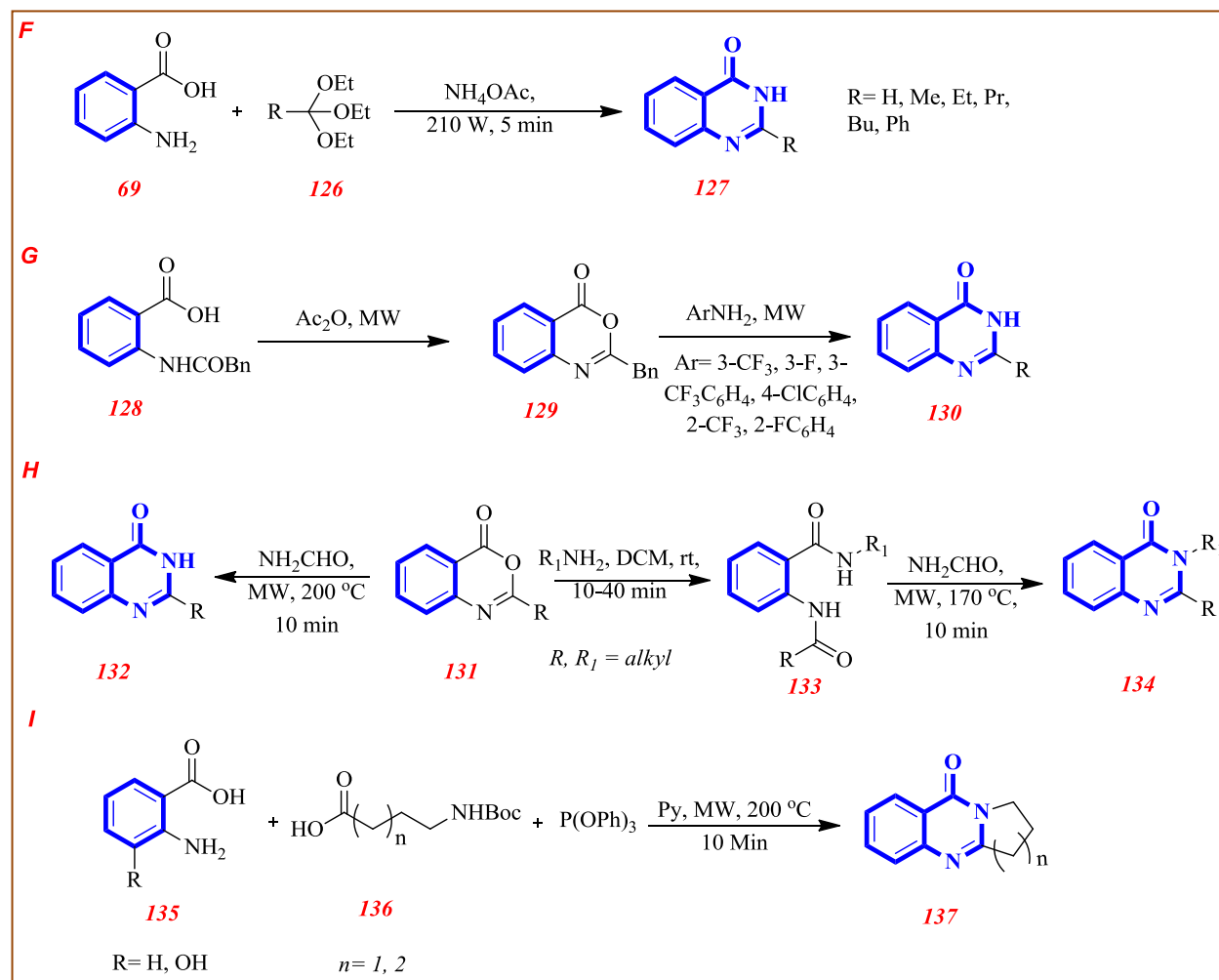
Eqn. 13. Synthesis of various quinazolinone via microwave
