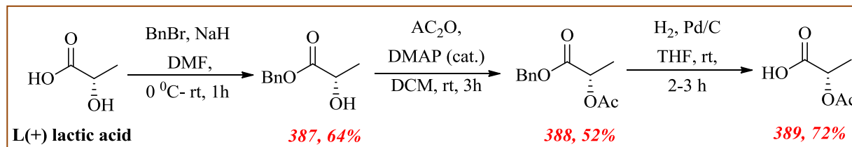
Scheme 26. Synthesis of (S)-2-acetoxypyranoic acid
