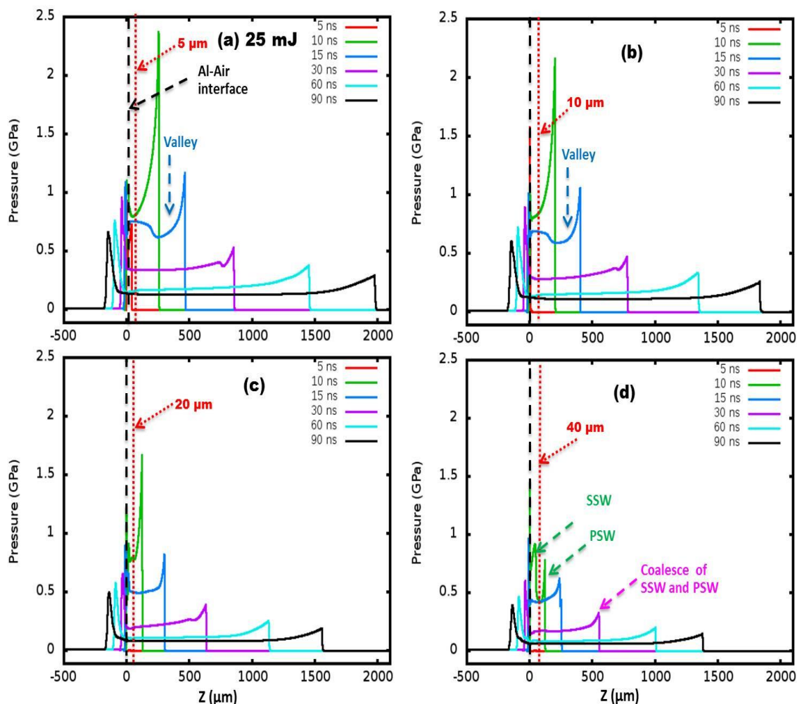
Figure 5.8 Comparison of numerically simulated pressure with varying separation D at a) 5\ \mu\text{m} b) 10\ \mu\text{m} , c) 20\ \mu\text{m} and d) 40\ \mu\text{m} for the input laser energy of 25\ \text{mJ} .
