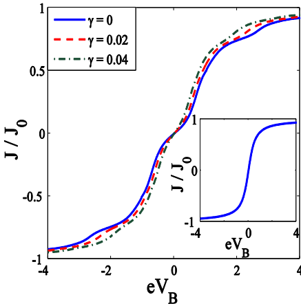
Fig. 2 J/J_0 as a function of eV_B with \lambda = 0.6 . (Inset: J/J_0 for \lambda = \gamma = 0 )
