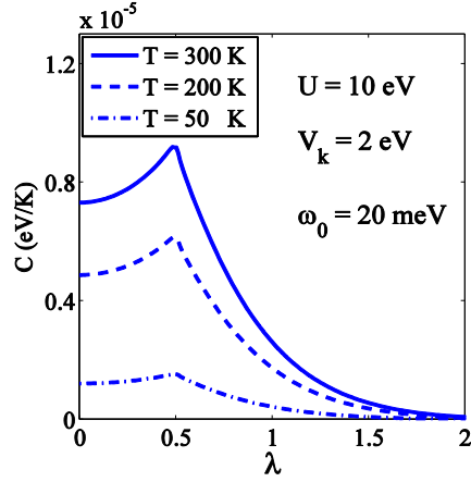
Fig. 8 C vs \lambda for different values of T .
